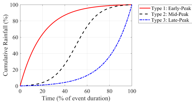
Figure 5. Schematic representation of rainfall event types based on the temporal distribution of cumulative rainfall. The x -axis represents the percentage of event duration, while the y -axis indicates the cumulative percentage of rainfall.
