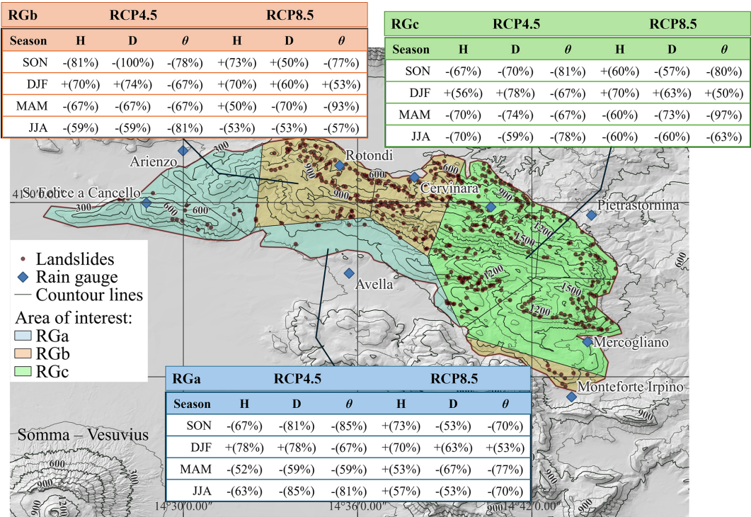
Figure 7. ubregional trend (positive “+” or negative “−”) and percentage of agreement (in brackets) of the ensemble members on rainfall ( H ), intensity ( D ) and antecedent volumetric water content ( \theta ), according to RCP4.5 and RCP8.5 climate change scenarios.
