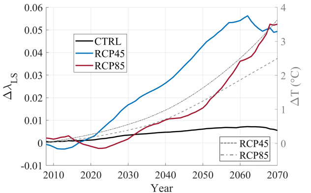
Figure 8. Anomalies on the trend component of the time series of temperature ( \Delta T ) and landslide frequency trend ( \Delta \lambda_{LS} ) in the study period under RCP4.5 (blue) and RCP8.5 (red) scenarios, based on climate model ensemble simulations. Temperature change ( \Delta T ) represents the anomaly relative to the 2006 baseline.
