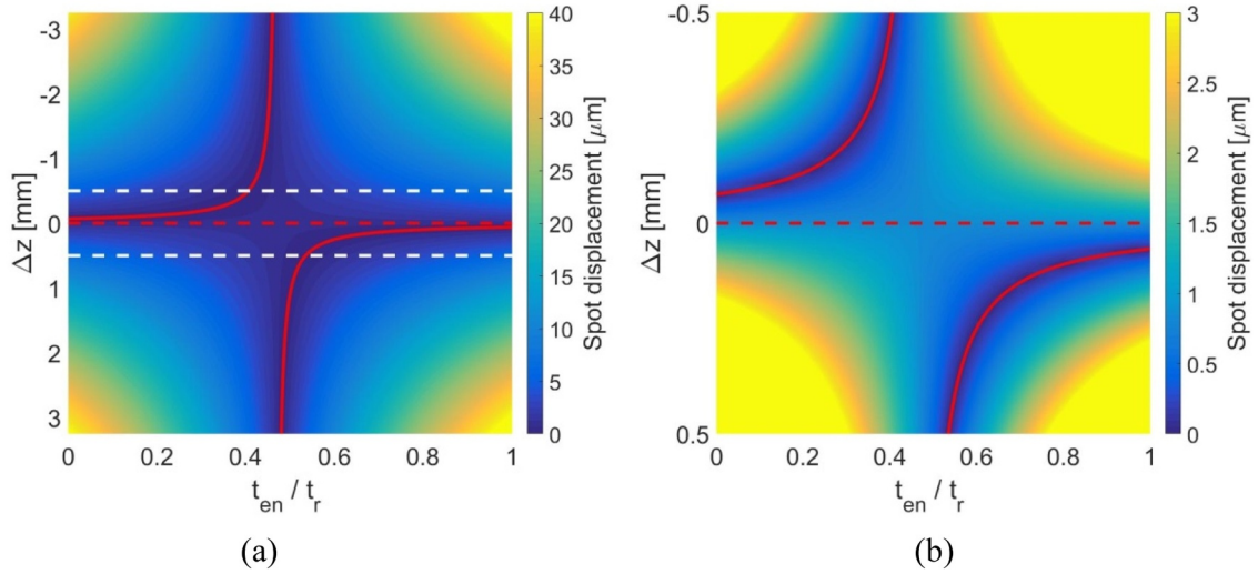
Fig. 4. (a) Spot displacement in between the blarker plates in relation to the relative arrival time in the blarker and the misalignment of the focus with respect to the blarker middle plane. The color map indicates the magnitude of the spot displacement. Calculations with parameters from Ref. [1], with 5 keV electron energy. The red curve in the figure represents the conditions for which the spot displacement equals zero. The dashed red line indicates where the spot displacement remains constant. The two dashed white lines indicate the region shown in (b). In (b), it can be seen that the spot displacement around the middle plane of the beam blarker is about 1 \mu\text{m} . (For interpretation of the references to color in this figure legend, the reader is referred to the web version of this article.)
