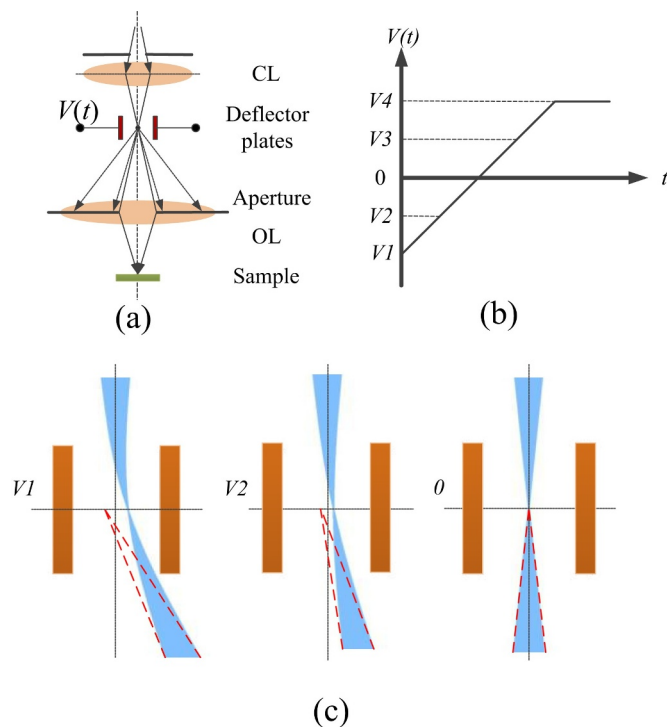
Fig. 1. (a) Schematic configuration of a blanking system with electrostatic deflector plates. A condenser lens (CL) focuses the beam in between the deflector plates. An aperture is positioned on the axis close to the objective lens (OL). The voltage input V(t) deflects the beam over the aperture generating an electron pulse. (b) Indication of an increasing voltage ramp with the beam deflection by the blanker at stages V1 , V2 , and 0 indicated in (c). In (c) the electron beam is indicated in blue and the apparent retraced focus spot position in the blanker is indicated in red. The magnitude of the resulting spot displacement depends on the arrival time of an electron in the blanker relative to V(t) . (For interpretation of the references to color in this figure legend, the reader is referred to the web version of this article.)
