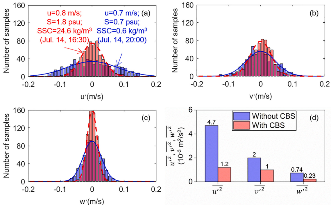
Fig. 12. Typical distributions of (a) streamwise ( u' ), (b) transverse ( v' ) and (c) vertical ( w' ) fluctuations of velocity and their Gaussian fits (curves) with (red) and without (blue) the presence of concentrated benthic suspension. (d) Comparison between the burst-averaged fluctuations under these two conditions. Data were collected at CS4T during the spring tide on 14 July 2014. PSU: practical salinity units. (For interpretation of the references to colour in this figure legend, the reader is referred to the web version of this article.)
