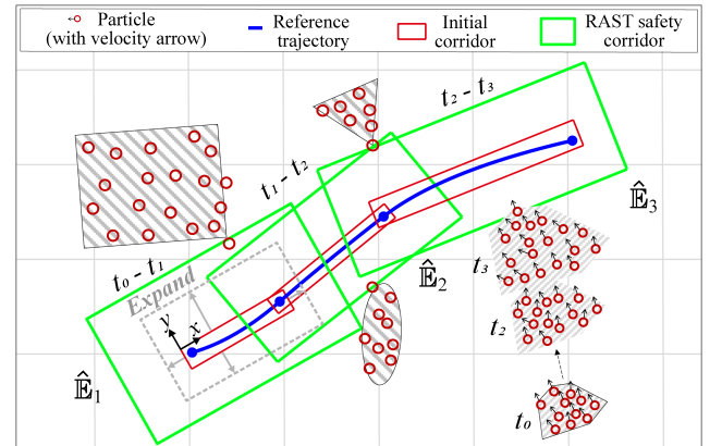
Fig. 6. Illustration of the safety corridor generation process. A three-piece reference path searched by the risk-aware kino-dynamic A* is shown with the blue curve. Red rectangles represent the initial safety corridors, which are then expanded to the RAST safety corridors \mathbb{E}_j . In the first RAST safety corridor \mathbb{E}_1 , a local coordinate is built on the initial corridor, and an intermediate state in the expanding is shown with a gray dashed box. The expansion is conducted to +x , -x , +y , and -y incrementally with different priorities.
