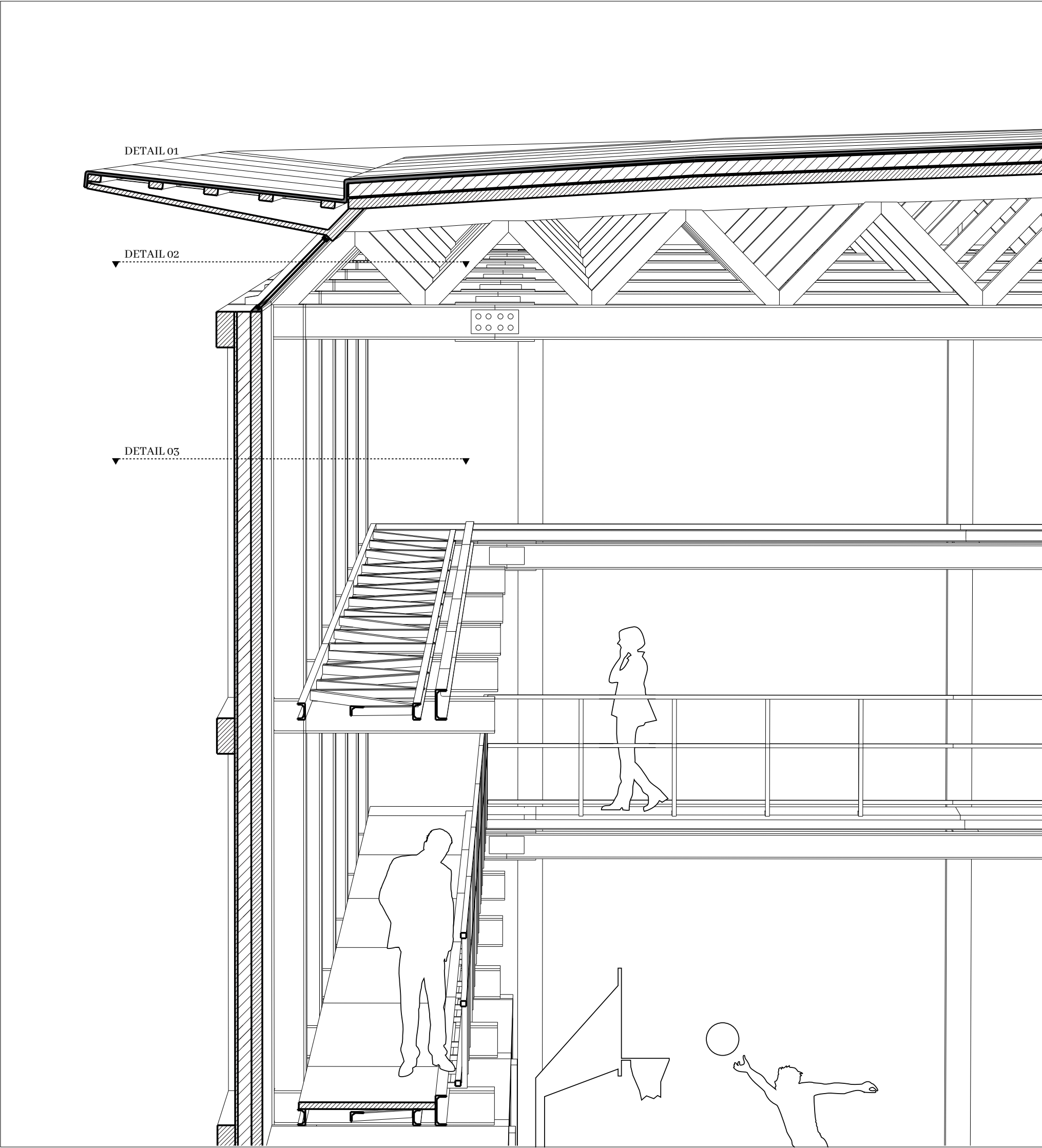
PERSPECTIVE DRAWING non-scale
