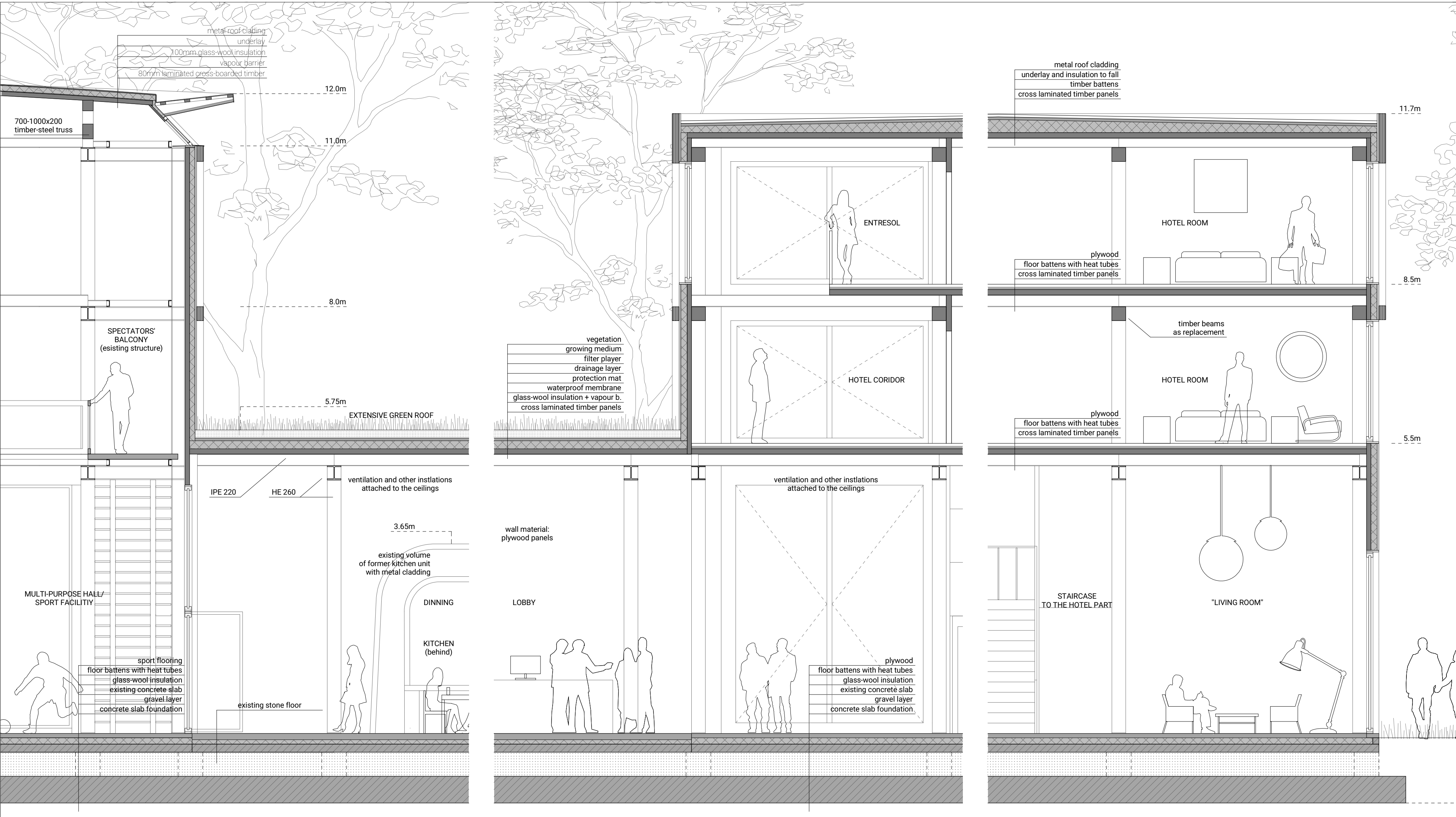
SECTION A-A' FRAGMENTS 1:50
