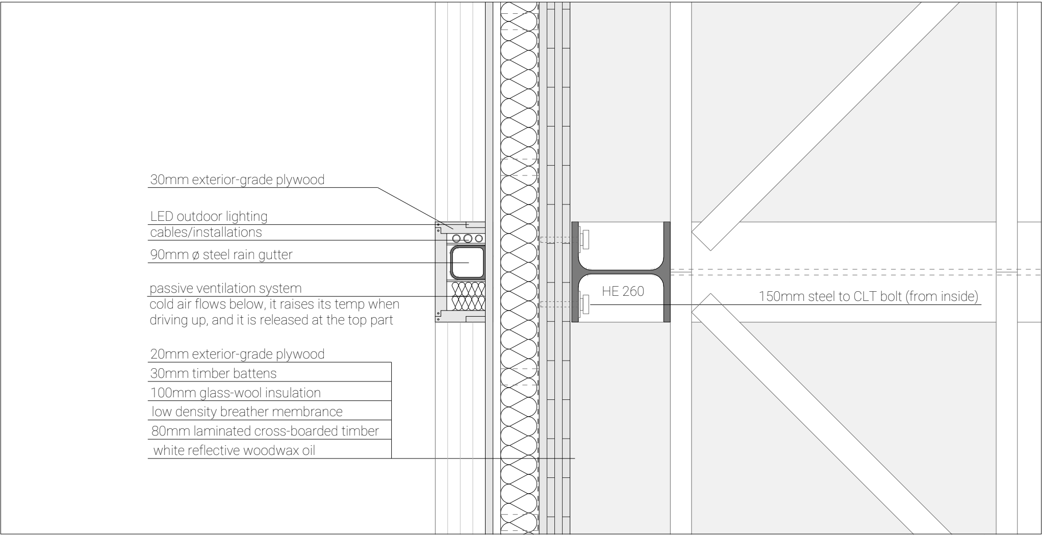
DETAIL 03 - horizontal cut B 1:10
