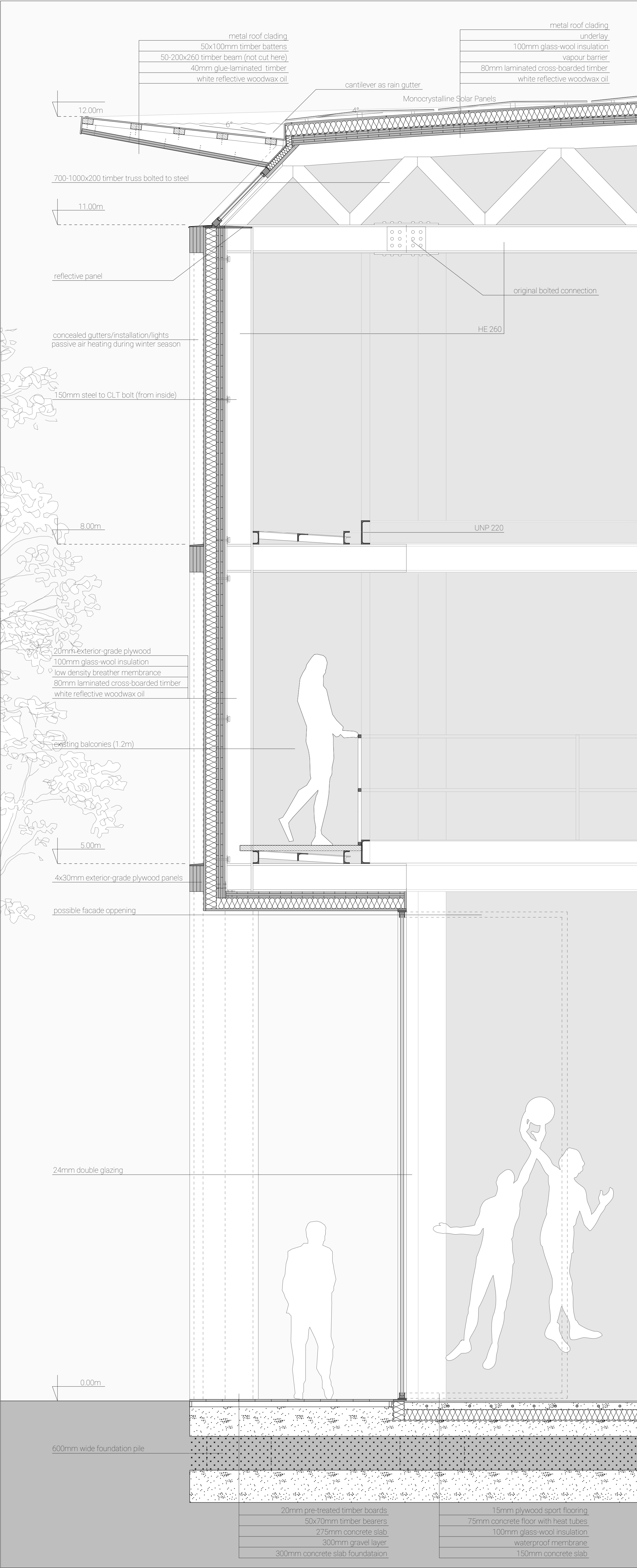
FAÇADE FRAGMENT - VERTICAL CROSS-CUT
