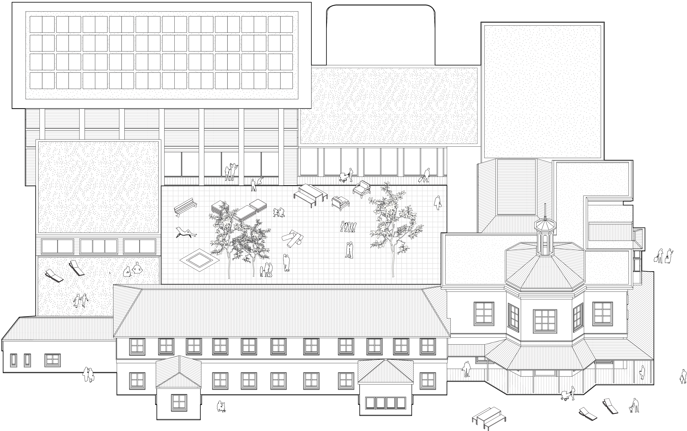
ISOMETRIC PROJECTION view from the South
