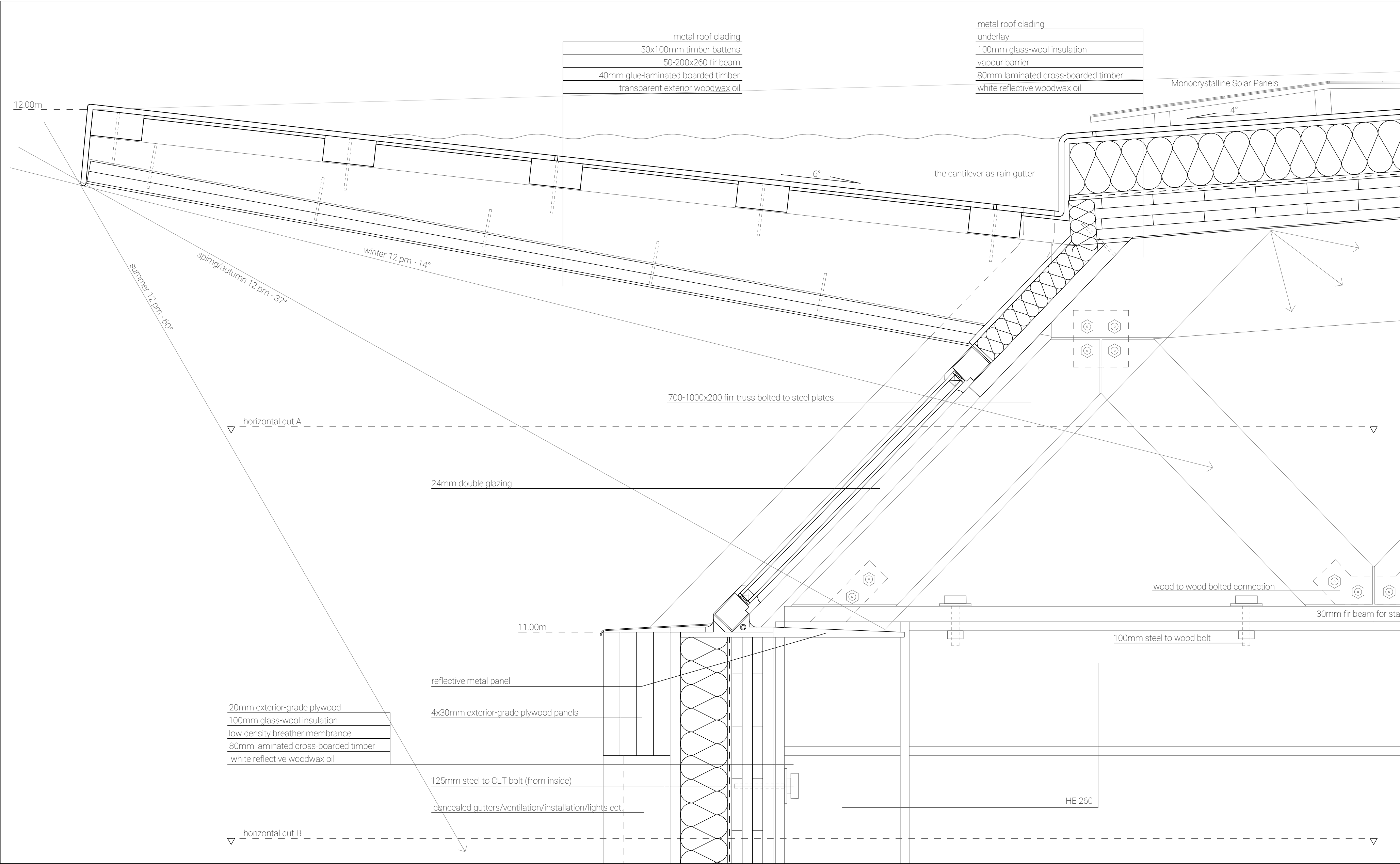
DETAIL 01 - vertical cut 1:5
