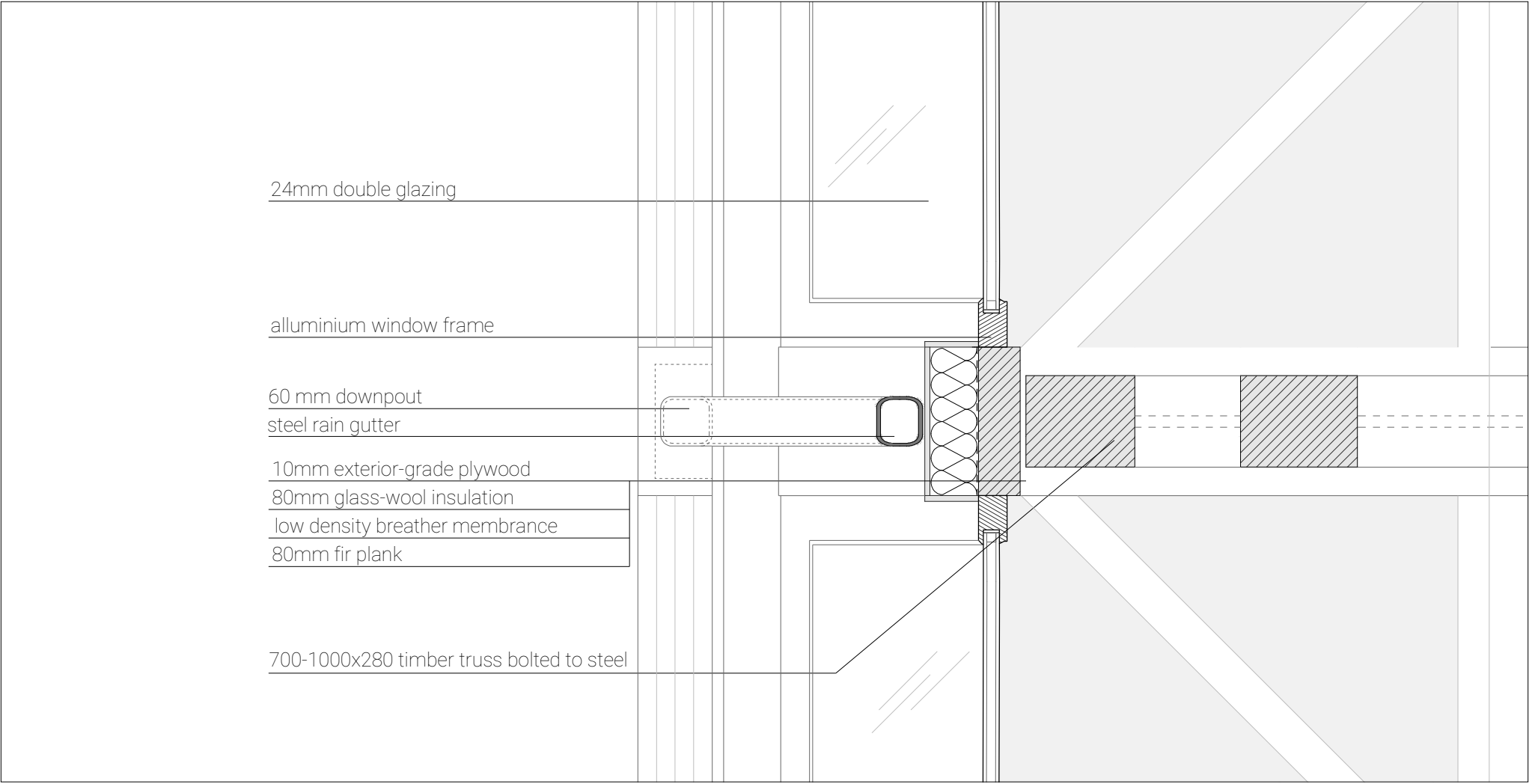
DETAIL 02 - horizontal cut A 1:10
