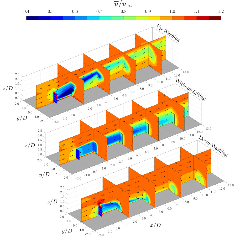
Figure 2. Contours of time-averaged streamwise velocity ( \bar{u} ) for cases UW-53 (top), WL-53 (middle), and DW-53 (bottom). Arrows are scaled by the square root of the in-plane velocity norm. The rotor part and lifting-devices of MRSL are represented by blue and red surfaces, respectively. The MRSL projection areas are outlined as squares in each x -plane.
