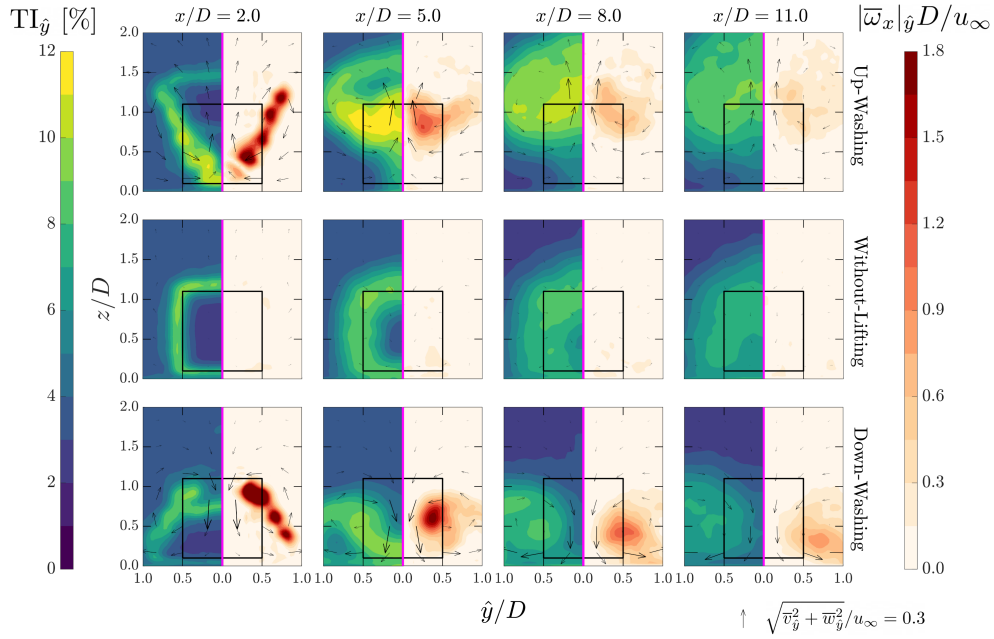
Figure 4. Contours of turbulence intensity (TI, left) and time-averaged streamwise vorticity ( \bar{w}_x , right) at different x -planes for cases UW-53 (top row), WL-53 (middle row), and DW-53 (bottom row). The x -planes are indicated at the top of each column. The subscript \hat{y} denotes averaging over the symmetry plane y/D = 0 (see Equation 4). Arrows' are scaled by the square root of the in-plane velocity's norm with their absolute scales provided in the bottom right.
