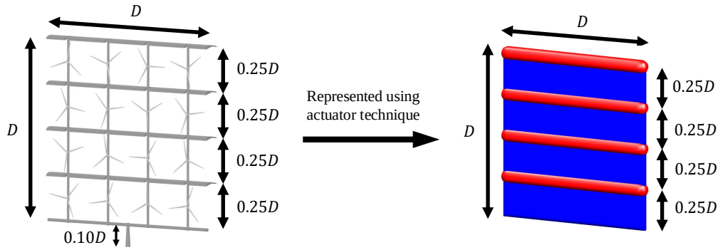
Figure 1. Left: A sketch illustrating how the multi-rotor system with lifting-devices (MRSL) could be in the real world. With the orientation of the wings, this MRSL is in Down-Washing configuration [7]. Right: MRSL represented with the actuator techniques. The rotor parts are parametrized as an actuator disk (blue surface). The lifting-devices/wings are degenerated into actuator lines (red surfaces). The key dimensions are labeled on both sides, with D being 300 m.
