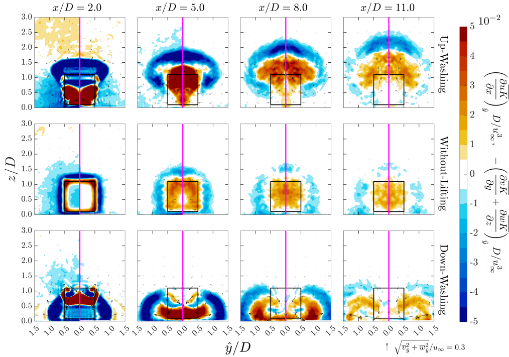
Figure 6. Contours of the energy equation's terms (Equation 5) for cases UW-53 (top row), WL-53 (middle row), and DW-53 (bottom row). The left of each panel plots the contour of \partial \overline{uK}/\partial x . The right plots the contours of -(\partial \overline{vK}/\partial y + \partial \overline{wK}/\partial z) . The x -planes are indicated at the top of each column. Arrows are scaled by the square root of the in-plane velocity's norm.
