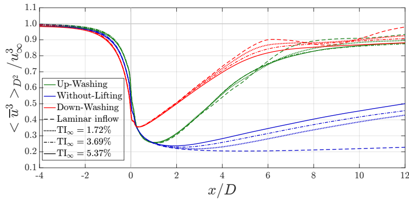
Figure 3. Area-averaged mean available power \langle \bar{u}^3 \rangle_{D^2} along the streamwise direction. The averaging area is the projection area of MRSL (see the black squares in Figure 2).
