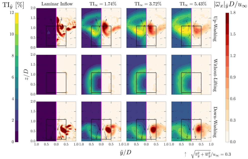
Figure 5. Contours of turbulence intensity (TI, left) and time-averaged streamwise vorticity ( \bar{w}_x , right) at x/D = 5 for cases with different TI_\infty , as indicated at the top of each column. The MRSL configurations shown in the top, middle, and bottom rows are UW , WL , and DW , respectively. The subscript \hat{y} denotes averaging over the symmetry plane y/D = 0 (see Equation 4). Arrows's length are scaled by the square root of the in-plane velocity's norm.
