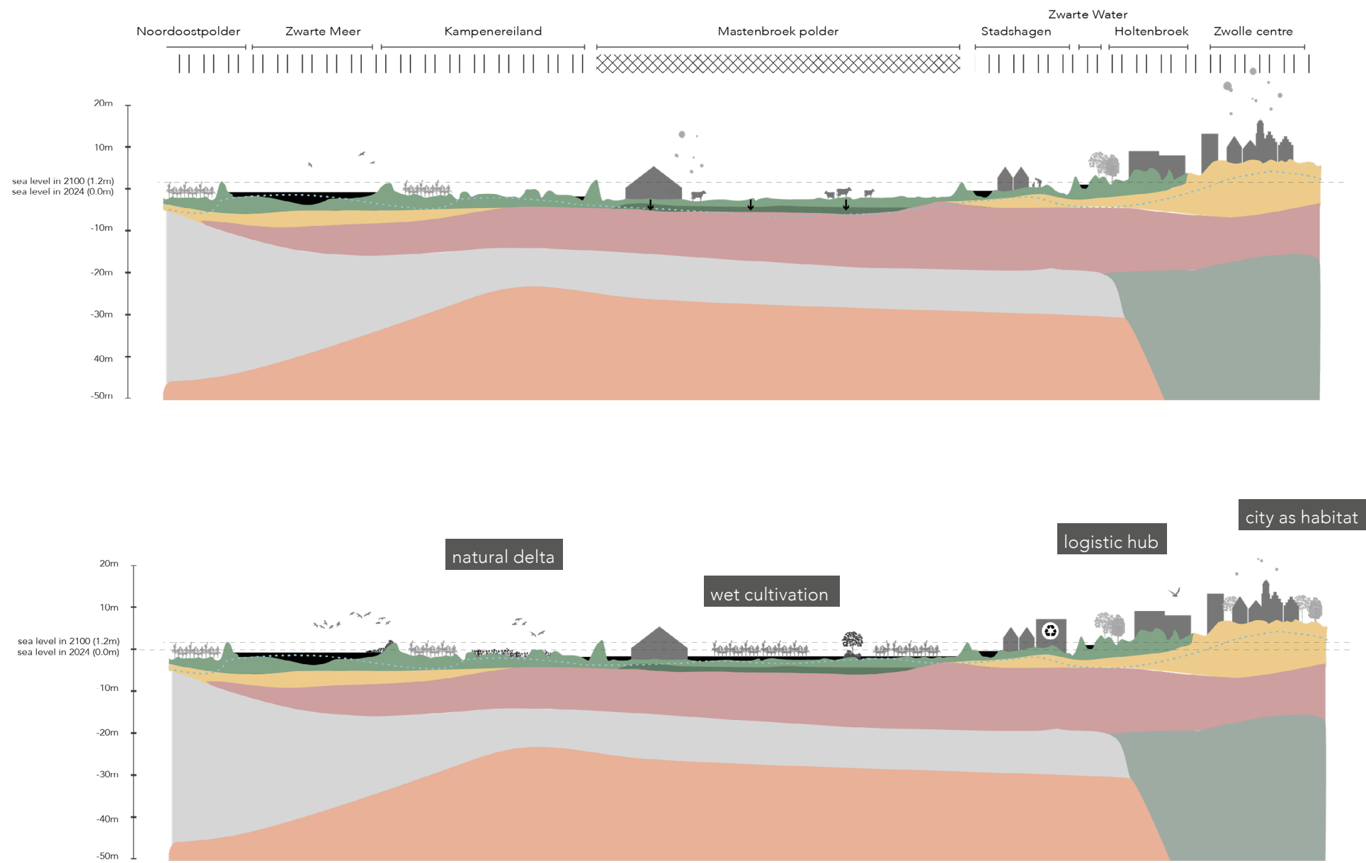
Top: section, current situation. Bottom: section, future vision
