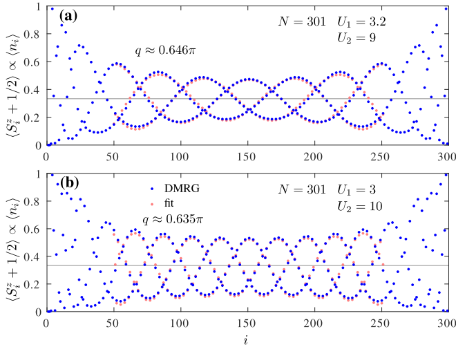
FIG. 5. Examples of the local density profiles inside the Luttinger liquid phase for large values of U_2 . Competition between the one-third filling constraint and next-nearest-neighbor interaction lead to incommensurate oscillations of the local density around the fixed value 1/3 (gray line). The DMRG data are shown in blue, the results of the fit are shown in pink, an incommensurate wave-vector q obtained from the fit is indicated at each panel.
