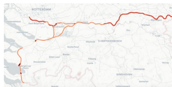
Figure 2 Overview map indicating large-scale patterns and hotspots of CO 2 emissions
