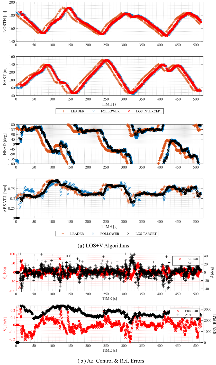
Fig. 7. Experimental model testing (wide-runs): controller setpoints and actuation. (a) LOS+V algorithms. (b) Az. control and ref. errors.
