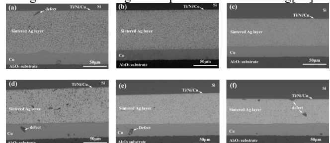
Fig.3 SEM images of cross-sections of the Si-Ag-DBC joints[12].
