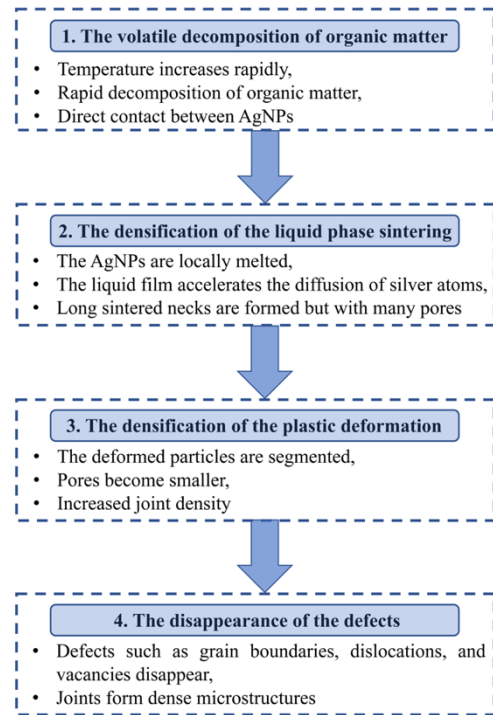
Fig.7 Schematic diagram of laser rapid sintering mechanism
