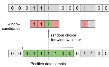
Fig. 5. Illustration of the process used to select positive laughter samples for our machine learning tasks. Given the binary laughter/non-laughter annotations for a particular segment, we select a location for the window center from the positively-annotated intervals in the signal. We then extract a window of 1.5 seconds around the chosen center. We pad if necessary.
