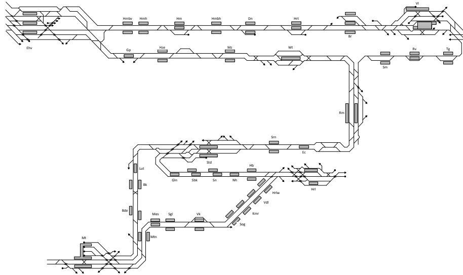
Figure 3: The schematic track layout of the considered network
