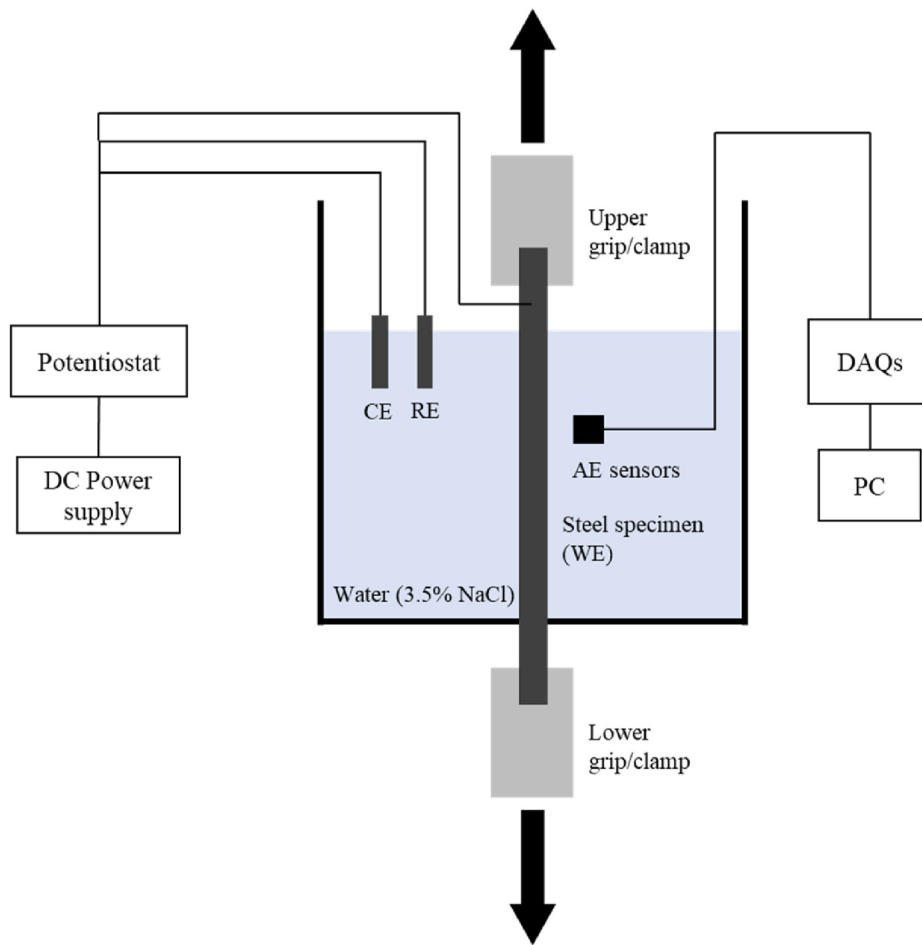
Fig. 3. Schematic illustration of the corrosion-fatigue test setup and instrumentation.
