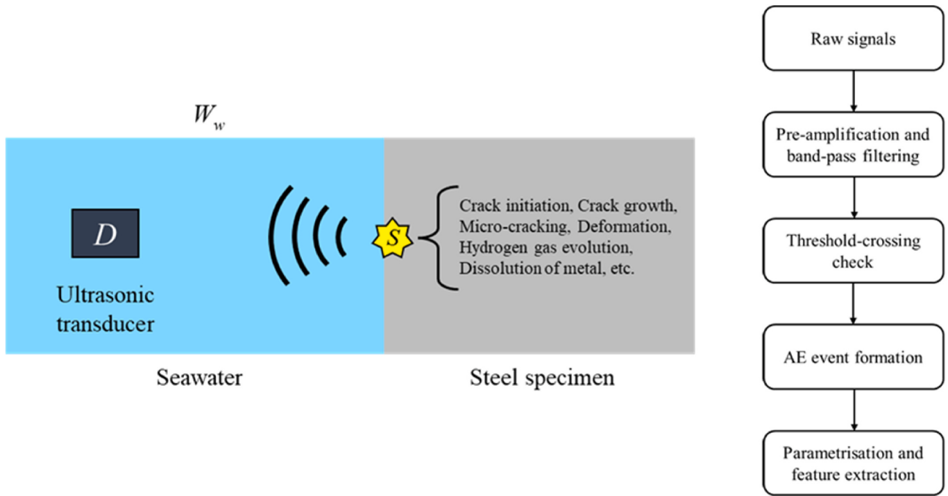
Fig. 1. Schematic illustration of underwater non-contact AE measurement (left) and signal analysis process (right).
