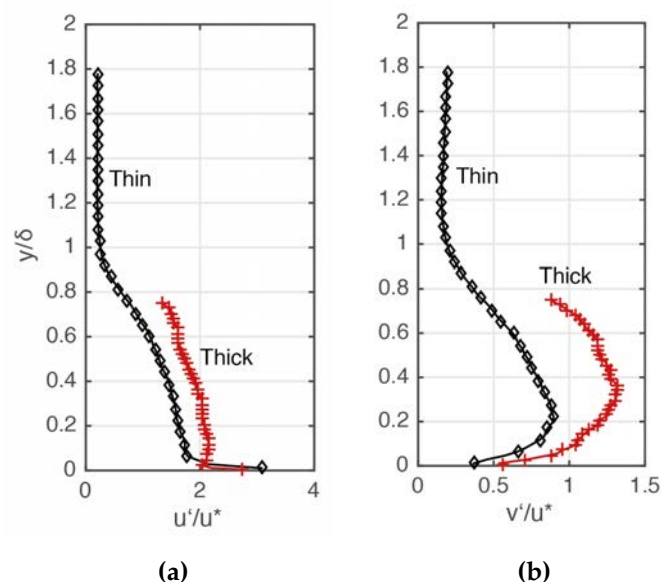
Fig. 7 Turbulence intensity profiles at the centre of the flat test plate and at Re_D \approx 40,000 . Every third data point is shown. Obtained using the panoramic PIV data.
