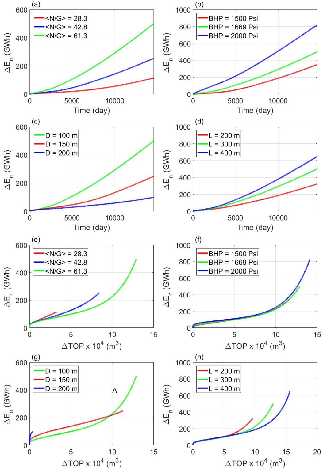
Figure 12: (a) – (d): Results of total consumed energy with time of simulation for a) various N/G s when D = 100 \text{ m} , L = 300 \text{ m} , BHP = 1669 \text{ Psi} b) various BHP when D = 100 \text{ m} , L = 300 \text{ m} , N/G = 61.3 \% , c) different wellbore spacing when L = 300 \text{ m} , BHP = 1669 \text{ Psi} , N/G = 61.3 \% , d) various wellbore lengths when D = 100 \text{ m} , BHP = 1669 \text{ Psi} , N/G = 61.3 \% . (e) – (h) show the results of total consumed energy versus \Delta TOP for the same scenarios as those mentioned in (a) to (d).
