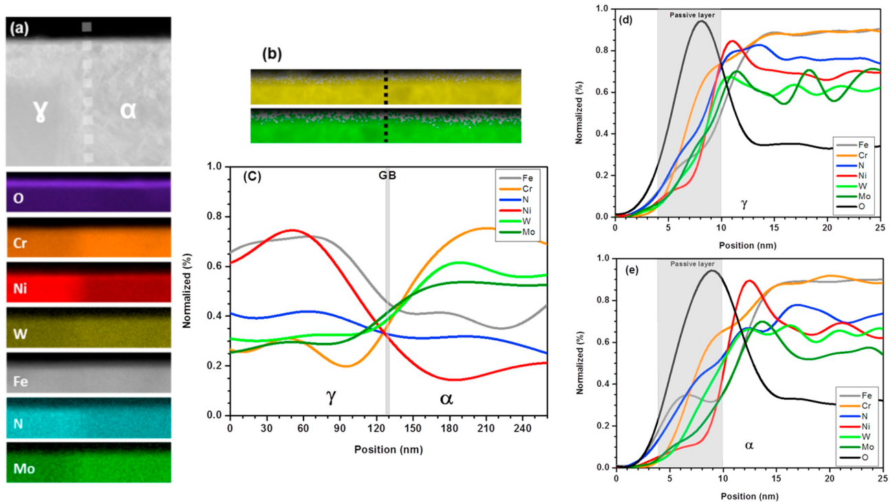
Fig. 3. (a) STEM image and EDS elemental maps, showing the distribution of alloying elements in austenite and ferrite. (b) Tungsten (top) and molybdenum (bottom) map superimposed on the STEM image to better show the element distribution within the passive layer. (c) Distribution of alloying elements in the passive film across the austenite/ferrite boundary (marked with line I in Fig. 2). The composition of passive layer is distinctly different from that in the bulk for both ferrite and austenite phases (Table 1). Cross sectional elemental profiles in (d) austenite (along line II in Fig. 2) and (e) ferrite (along line II in Fig. 2). As the border between the inner and outer passive layer is not sharp, the schematically shown passive layer is not divided into two sections.
