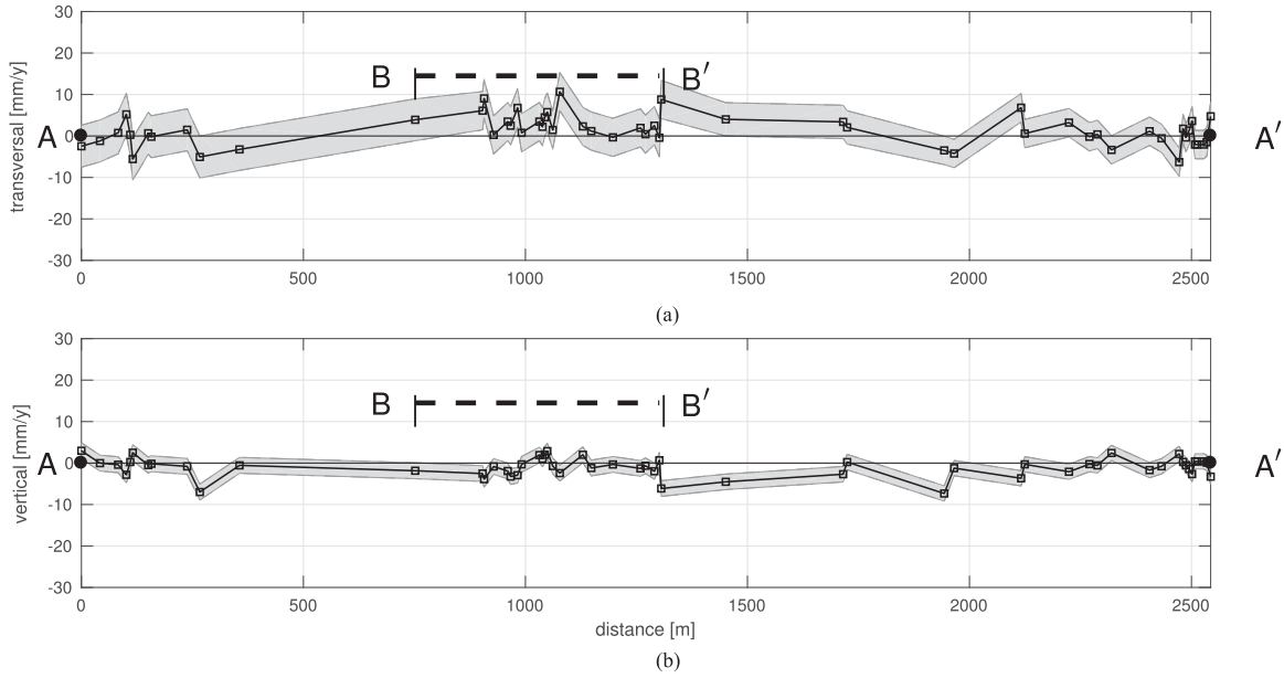
Fig. 11. LOS-vector decomposition results for the Rijpwetering railway segment A-A' as shown in Fig. 10. (a) Deformation velocity in the transversal direction. The positive sign indicates a movement towards the East. (b) Deformation velocity in the vertical direction. The black squares represent the velocity estimators (a) \hat{d}_T and (b) \hat{d}_N for the point-pairs, with the uncertainty shown in gray.
