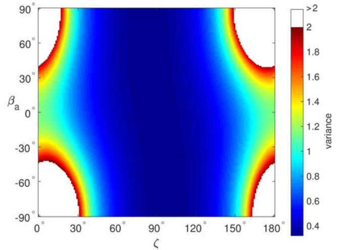
Fig. 5. Variance \sigma_{\hat{x}_p(\beta_a, \zeta)}^2 of the unknown parameter \hat{x}_p(\beta_a, \zeta) , given both Envisat and Radarsat-2 data in ascending and descending orbit. The x-axis represents the orthogonal elevation angles \zeta of a unit deformation vector, while the y-axis represents the asset azimuth angles \beta_a of the line-infrastructure.
