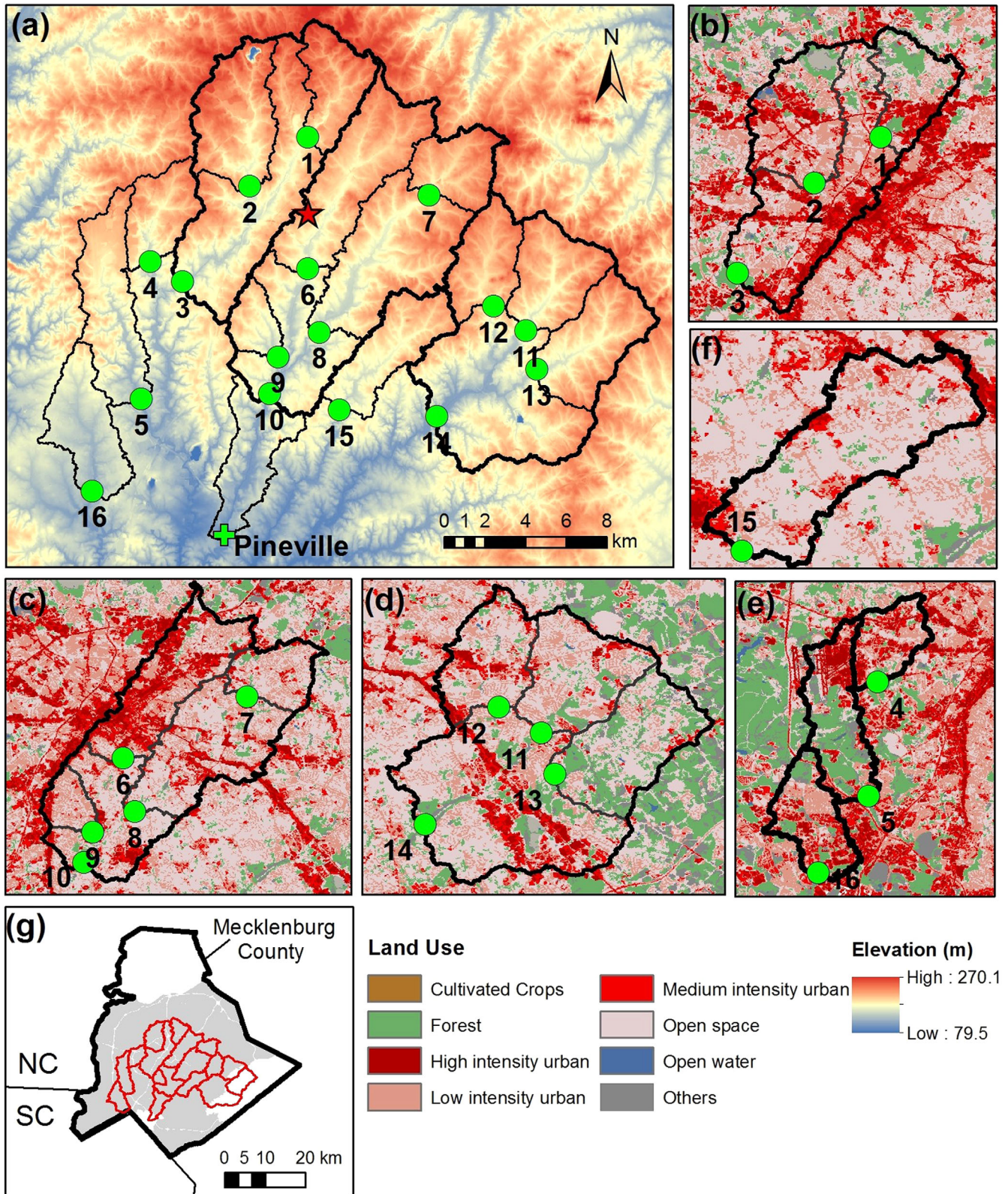
Figure 1. Location map for the Charlotte study area, with watershed boundaries and land use/land cover. The numbers of watershed are the same as those in Table 1. (a) The red star is denoted as urban core, which is located in No.6 with the largest imperviousness. (g) The black outline is the boundary of Mecklenburg County, NC and the grey area is the city of Charlotte.
