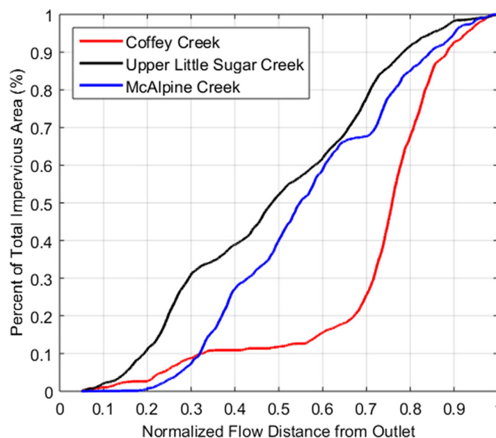
Figure 2. Distribution of impervious area as a fraction of distance from the basin outlet of Coffey Creek (No.5), Upper Little Sugar Creek (No.6), and McAlpine Creek (No.14).
