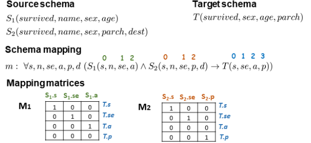
Figure 1: Schema mapping and mapping matrices
