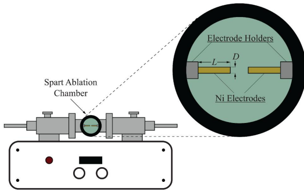
Figure 1. Schematic illustration of the SDG (VS-Particle, Model G1), including details of the configuration of the electrodes, employed in our experiments.
