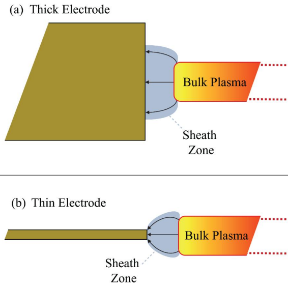
Figure 6. Illustration of electric field lines near the cathode for the cases where the diameter of the cathode electrode is larger (a) or smaller (b) than that of the bulk plasma. The region between the plasma and the electrodes is a sheath zone within which the ions are accelerated toward the cathode electrode.
