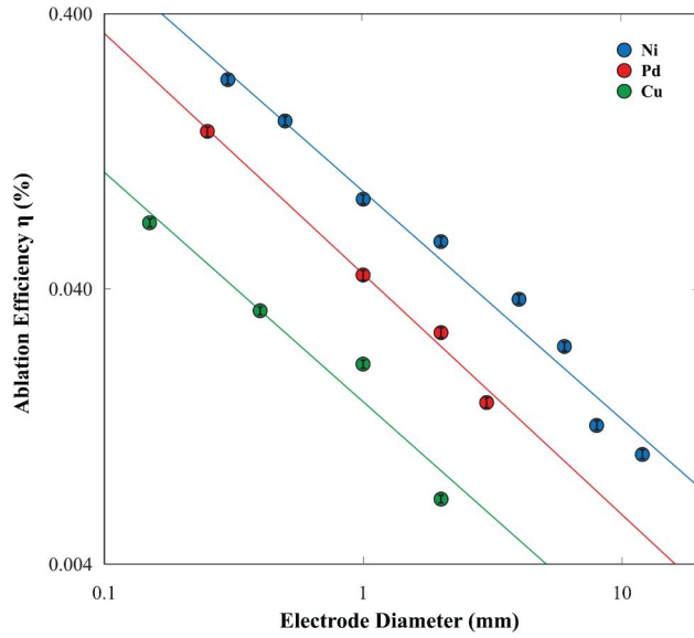
Figure 3. Ablation efficiency, \eta , as a function of the electrode diameter for the three materials studied in this work. The ablation efficiency is determined by Equation (3), using ablation and total energies determined by the experiments.
