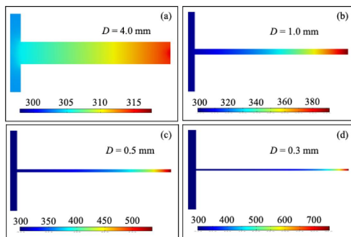
Figure 4. Temperature distributions along Ni electrodes of different diameters employed in the SDG, determined by the COMSOL simulations (a)–(d), and temperature difference between the front and back of the electrodes, or the carrier gas and the surface of the electrodes induced respectively by conduction or convection, as a function of the electrode diameter (e).
