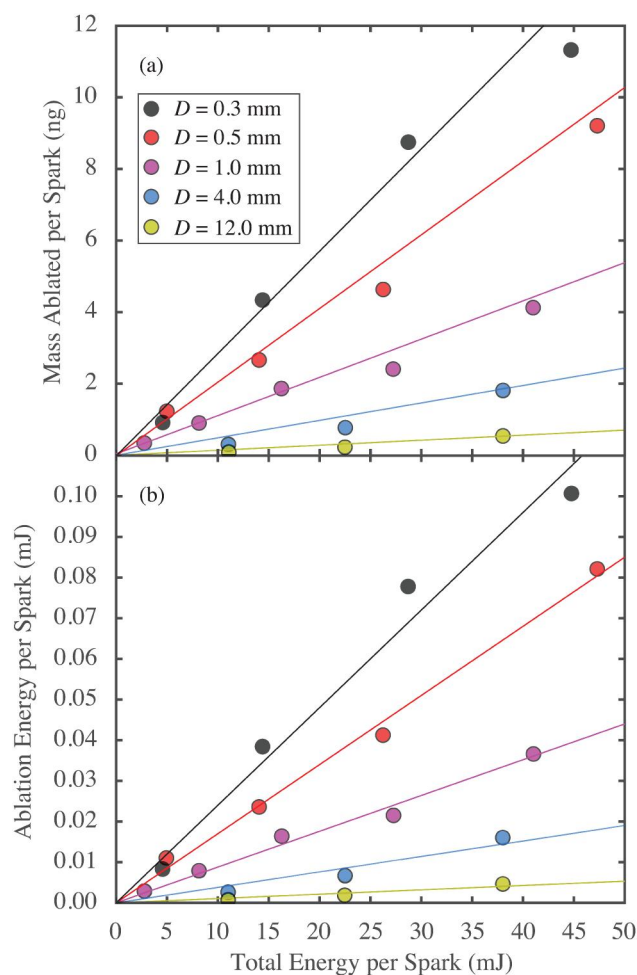
Figure 2. Results from gravimetric measurements corresponding to different diameters of Ni electrodes expressed as: (a) mass ablated from the electrodes as a function of the total electrical energy per spark provided to the SDG, and (b) fraction of input energy going to ablation, determined as the slopes of the fitted curves in the top sub-plot. The flow rate and spark frequency in these measurements were kept constant at 10 L/min N_2 and \sim 200 \pm 20\text{ Hz} .
