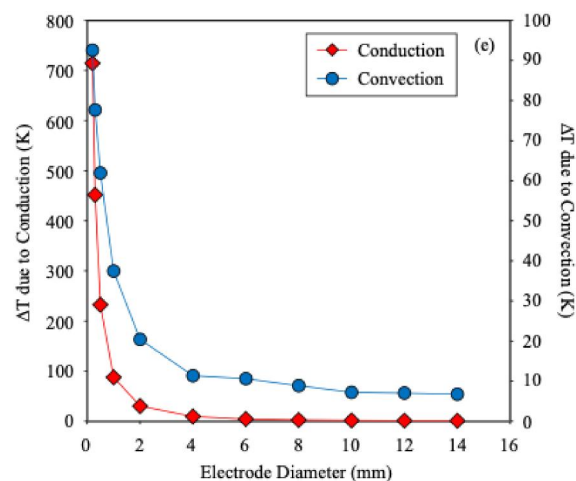
Figure 4. Temperature distributions along Ni electrodes of different diameters employed in the SDG, determined by the COMSOL simulations (a)–(d), and temperature difference between the front and back of the electrodes, or the carrier gas and the surface of the electrodes induced respectively by conduction or convection, as a function of the electrode diameter (e).
