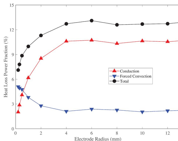
Figure 5. Fraction of input power lost as heat due to conduction and convection within the SDG chamber, determined by the COMSOL simulations.
