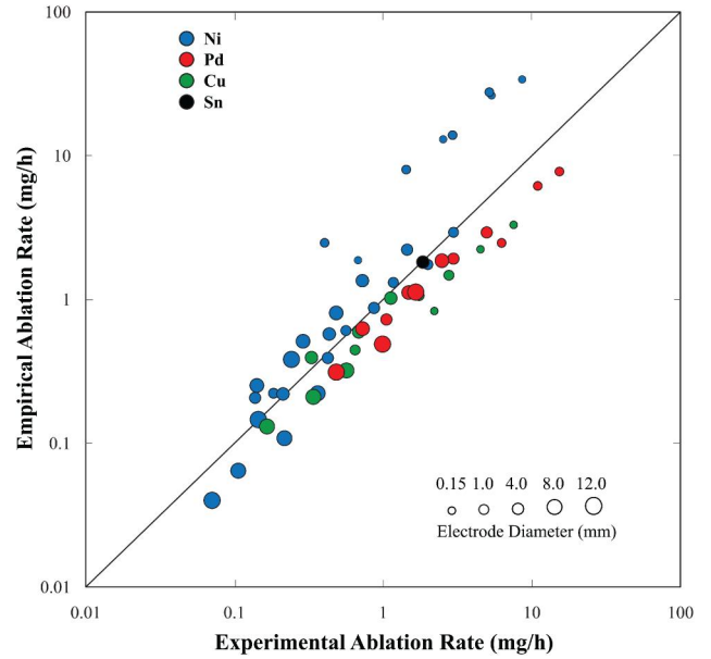
Figure 7. Correlation between the ablation efficiency determined by the experiments (values in the x axis) and by the simplified scaling law relating it with the diameter of the electrodes (values in the y axis) for all the materials tested in this work. The size of the circles indicates the diameter of the electrodes, ranging from 0.15 to 12 mm.
