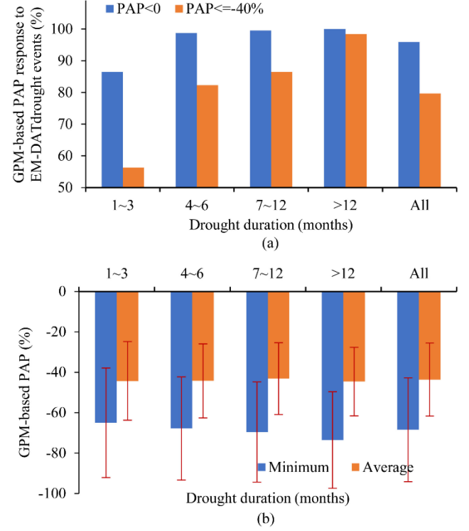
Fig. 3. (a) Percentage of GPM-based PAP response to drought events from the EM-DAT database. (b) Average and minimum of PAP.
