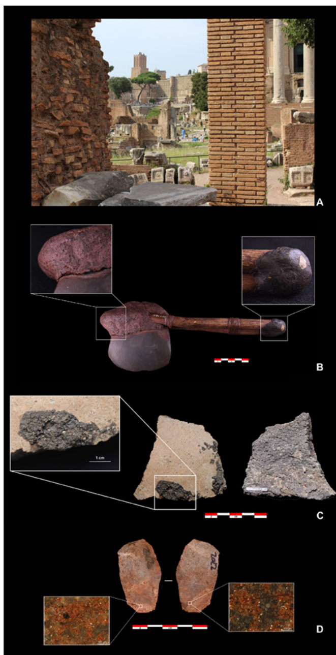
Figure 1. Examples of different adhesives. A , Roman concrete at the Forum Traiani in Rome (Italy). In the background, Trajan's Market (100–110 CE) and the Tower of the Militia (13th century CE). The walls and the pillars in the foreground are built in opus latericium , which was the predominant construction technique in the Imperial Era. In the brick wall on the left, the facing is missing and the concrete core ( opus caementicium ) is clearly visible. B , Ethnographic Australian aboriginal axe hafted with spinifex resin adhesive mixed with ochre and plant fibers. C , Pre-Columbian ceramic sherd with black adhesive remains relating to pottery repair, from the La Cajita site in Colombia, dating to about 1230 CE. D , Dorsal and ventral view of a weathered experimental flint tool with ochre stains resulting from the ochre-loaded hafting adhesive (Kozowyk, van Gijn, and Langejans 2020). Photos courtesy of Maria Pina Garaguso ( A ), Paul Kozowyk ( B ), and Alessandro Aleo ( C , D )
