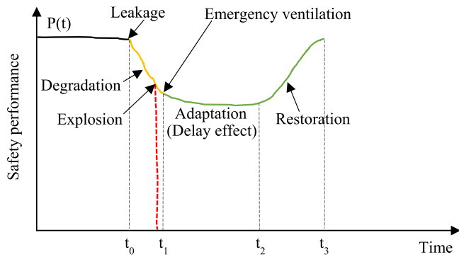
Fig. 9. A schematic safety performance curve of the natural gas compartment.
