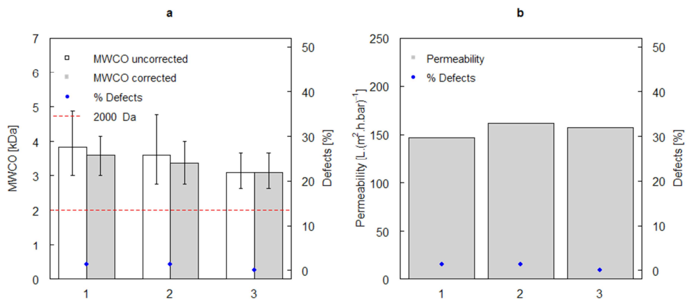
Figure 8 (a-b): MWCO in kDa (a) and hydraulic permeability in L \cdot (m^2 \cdot h \cdot bar)^{-1} (b) of pristine ceramic tUF membranes. MWCO of disc membranes with a purchased cut-off of 2 kDa (dashed line) was calculated without (white bars) and with correction for defects (grey bars). The percentages of defects in the membrane are shown (dots). The error bars represent the standard deviation of triplicate measurements. One batch is shown.
