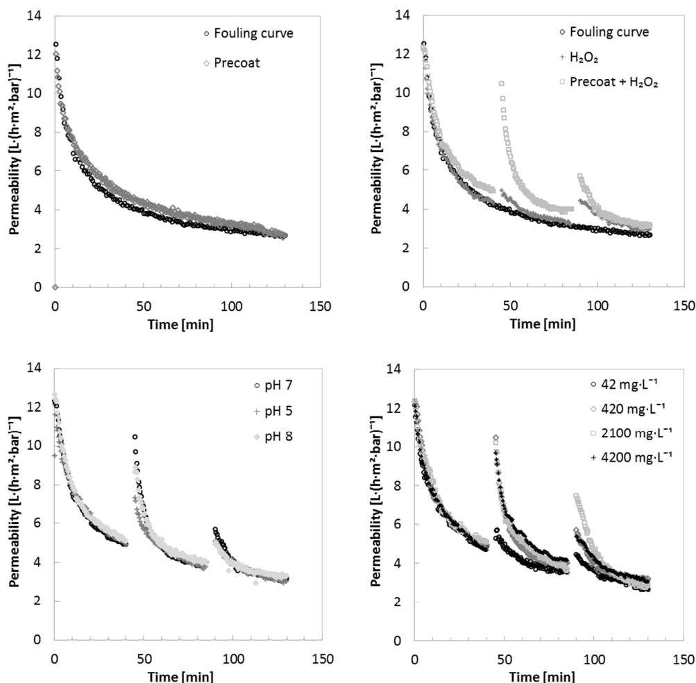
Figure 3a-d: Permeability in time of ceramic NF using model sewage using (a) untreated and iron chlorite precoated membranes. (b) Comparison of hydrogen peroxide cleaning on an untreated and precoated membrane. (c) Comparison of precoating suspensions of pH 5, 7, and 8. (d) Comparison of different precoating suspension concentrations.
