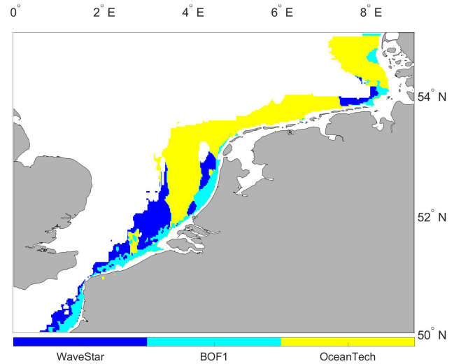
Fig. 5. Spatial distribution of "optimal" WECs for the domain.
