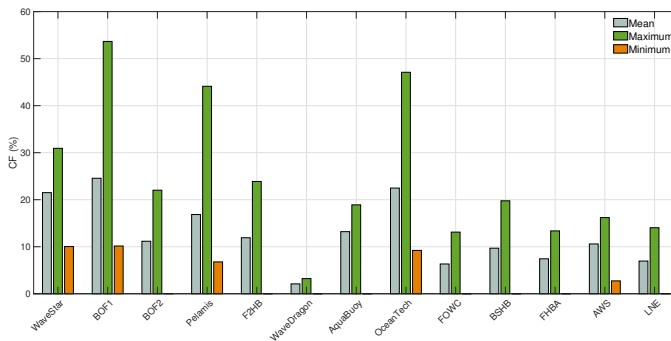
Fig. 3. Power performance indicator for all WEC devices, spanning from 1980-2017.
