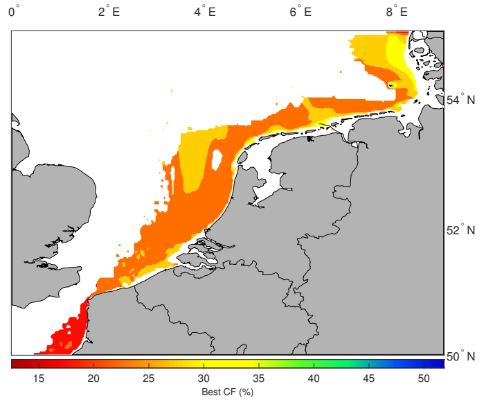
Fig. 4. Attained CF at the active locations, regardless of WEC, all options have been assessed simultaneously.
