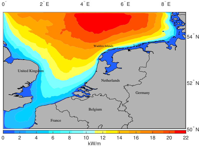
Fig. 2. Wave energy flux in the North Sea region, the dataset is based on North Sea Wave Database (NSWD) presented in [40], spanning from 1980-2017.
