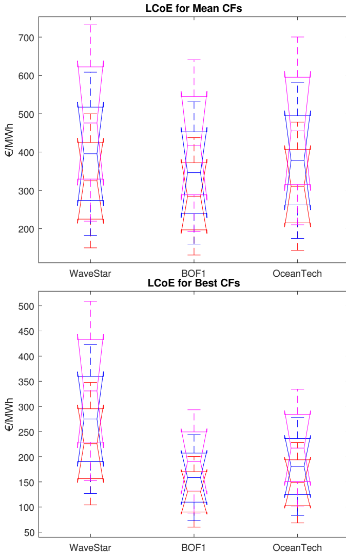
Fig. 6. LCoE distribution considering all CapEx ranges (1-5 million €) and the three discount rate scenarios with red 5%, blue: 10%, magenta 15%.
