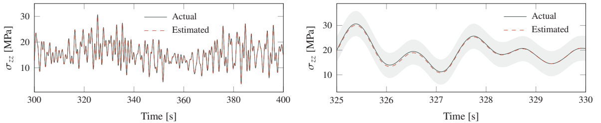
Figure 7: Actual and estimated stress time history with 95% confidence interval for location 2
