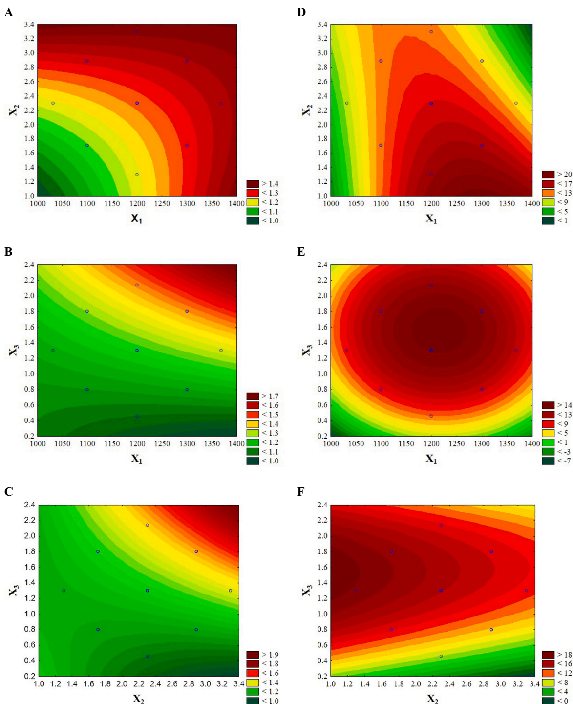
Fig. 6. 2D contour plots of the operating variables for the comparison and visual optimisation of the response variables: (A–C) H_2/CO molar ratio, (D–F) \eta_{solar \text{ to fuel}} ; X_1 = temperature, X_2 = H_2O/OPEFB molar ratio, X_3 = OPEFB flowrate.
