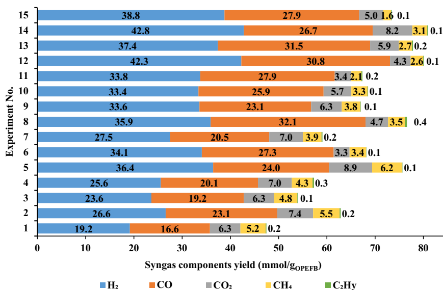
Fig. 2. Syngas yield and products composition for solar gasification of OPEFB under various operating conditions: Temperature (1100–1300 °C), H 2 O/OPEFB molar ratio (1.7–2.9), and OPEFB flowrate (0.8–1.8 g/min).
