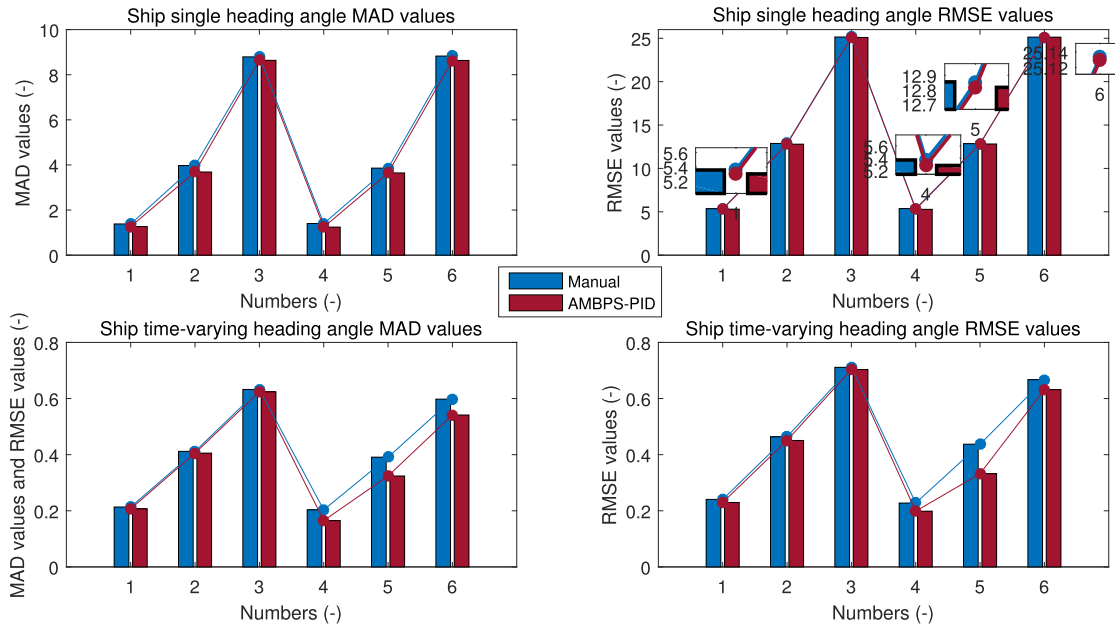
FIGURE 17. Tracking RMSE and MAD for ship control single heading angle and time-varying heading angles.
