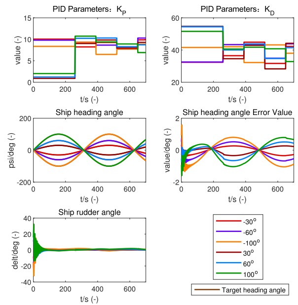
(b) Ship tracking details.
