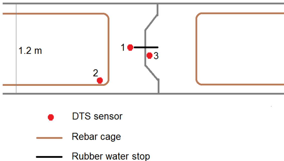
Figure 9: Cross section with DTS sensors relative to joint and rebar cages as applied during the field tests in Rotterdam
