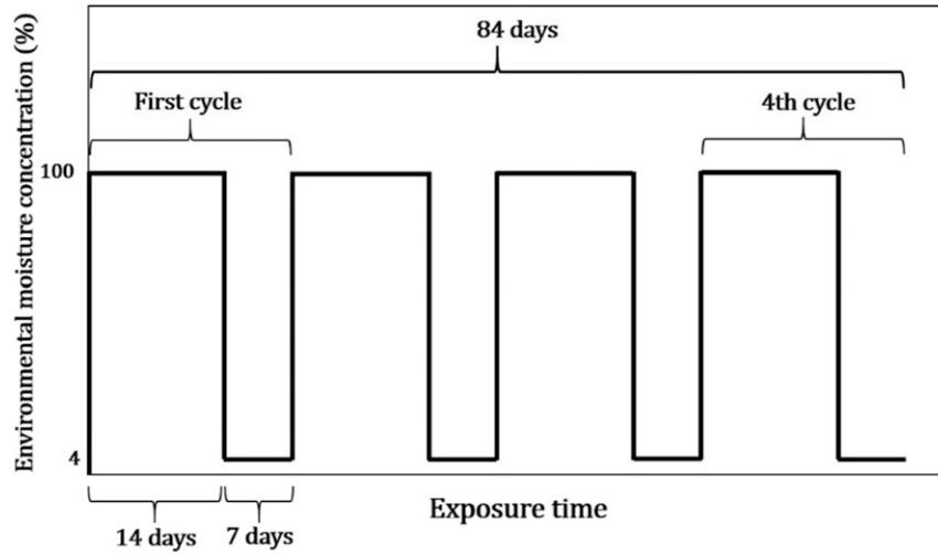
Figure 3. Schematic of the 14-day wetting/7-day drying cyclic aging process.
