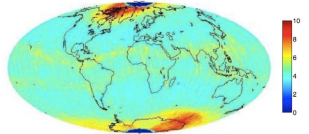
Figure 10. Global distribution of the RMS of the reduced-dynamic PSO phase residuals in (mm) for 2010.
