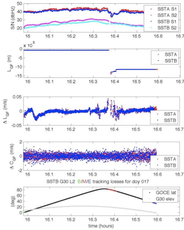
Figure 5. Analysis of several GOCE GPS tracking observables for G30 on 17 January 2011 using the main (SSTA) and redundant (SSTB) receiver.
