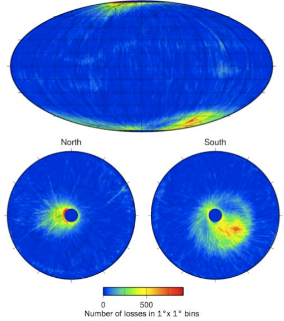
Figure 3. Distribution of unexpected L2 losses occurring in the middle of a pass in global view (top) and near the poles (bottom). Results are given in 1^\circ \times 1^\circ bins using almost 20 months of GOCE data.
