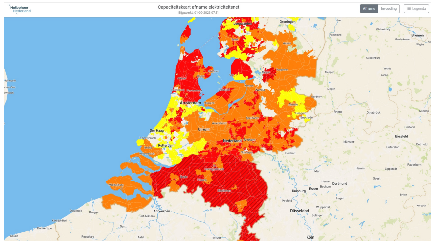
Figure 1.2: Map of congested areas for consumption in the Netherlands. Source: Netbeheer Nederland, 2023. No color: “transport capacity available”, yellow: “limited transport capacity available”, orange: “No transport capacity available for the time being pending the outcome of the congestion management study”, red: “No transport capacity available: congestion management cannot be applied”, red shaded: “no capacity available, congestion management fully used”.
