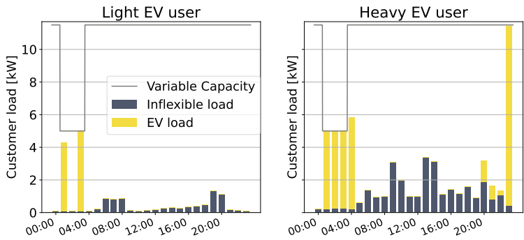
Figure 5.4: Day-ahead variable capacity limitation for flexible load in example day.
