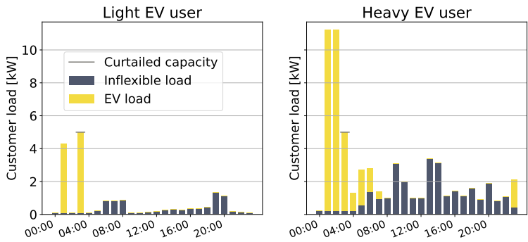
Figure 5.3: Interruptible connection in example day. Same users as in Figures 5.4 and 5.5.
