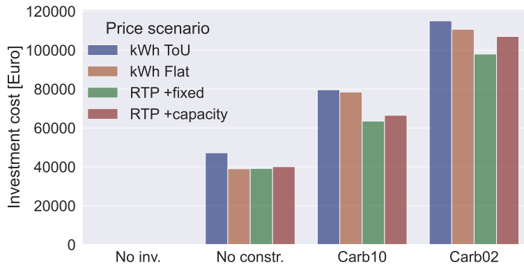
Figure 6.10: User investment costs of different rate designs and carbon constraints
