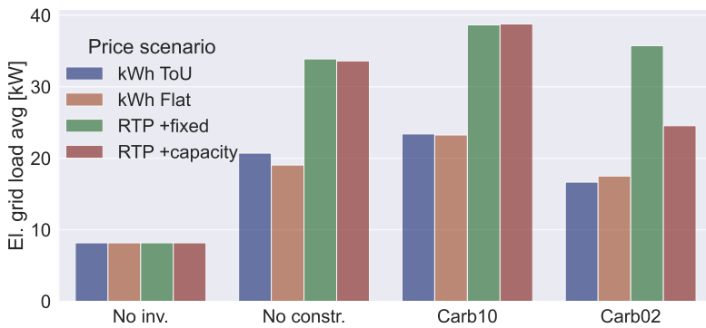
Figure 6.14: Average electric load of different rate designs and carbon constraints
