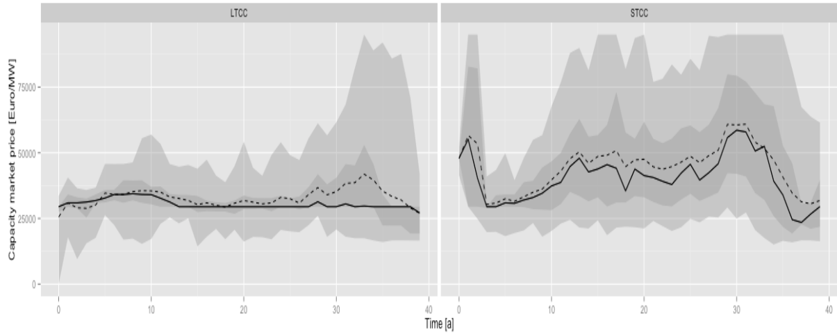
Figure 5.8: Capacity prices in scenario with a forward capacity market (left) and with a yearly capacity market (right).
