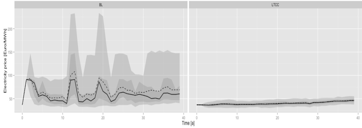
Figure 5.6: Electricity price in scenario without (left) and with (right) forward capacity market.
