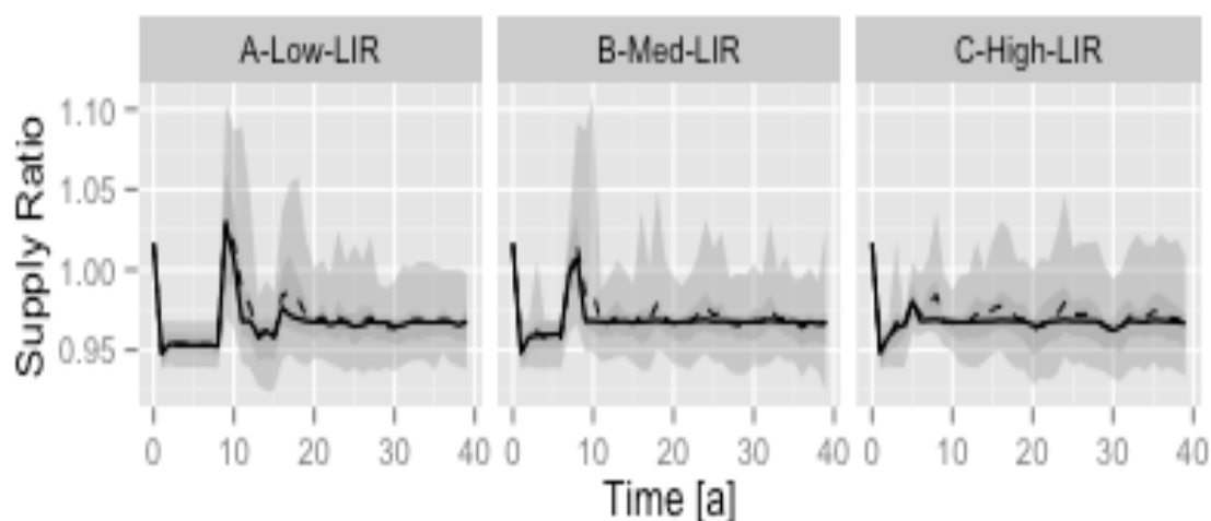
Figure E.2.1: Supply-ratio for scenarios with different interest rates.
