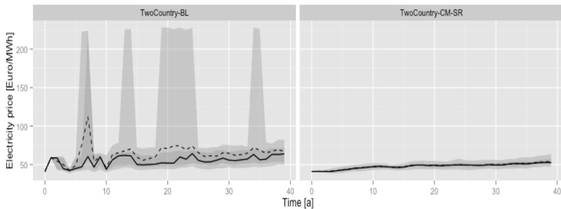
Figure 6.12: Electricity prices in the baseline (left) and in CM-SR scenario (right) in Zone A
