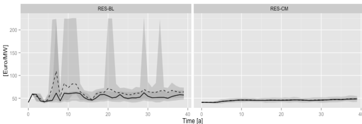
Figure 4.7: Electricity price in scenarios with growing share of renewables without (left) and with a capacity market (right)
