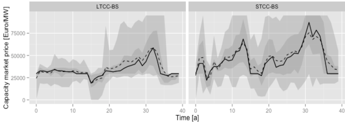
Figure 5.11: Capacity market prices in scenario with a forward capacity market (left) and a yearly capacity market (right)
