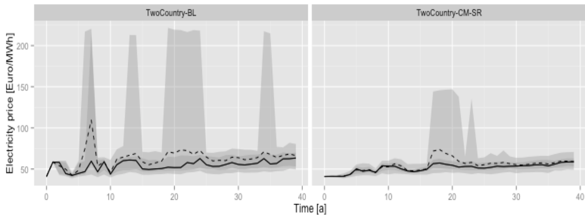
Figure 6.14: Electricity prices in the baseline scenario (left) and in scenario CM-SR (right) in Zone B
