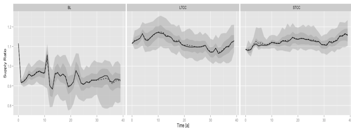
Figure 5.3: The supply ratio in scenarios without a capacity market (left), with a forward capacity market (center) and a yearly capacity market (right).
