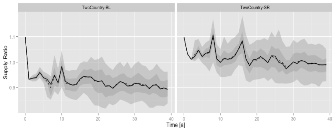
Figure 6.2: Comparison of supply ratio in Zone A without (left) and with a strategic reserve implemented.
