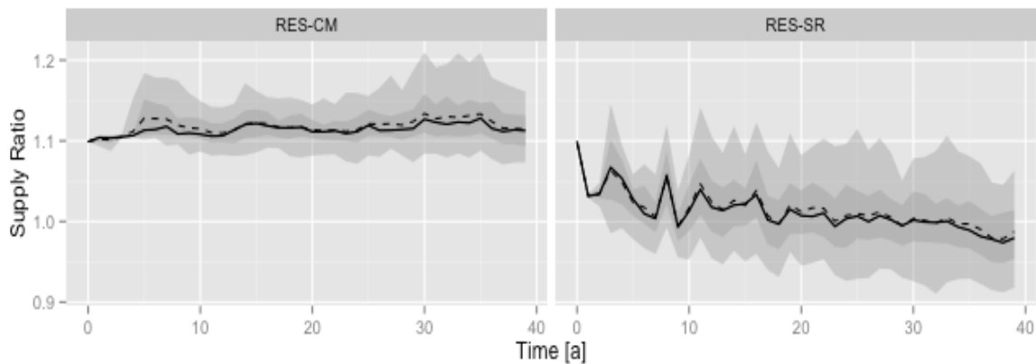
Figure 4.12: Supply ratio in the growing share of renewables with a capacity market (left) and with a strategic reserve (right).
