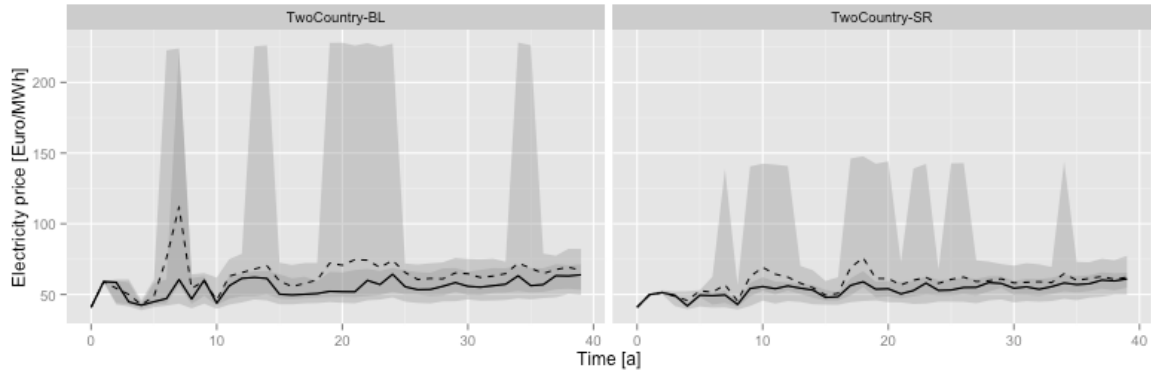
Figure 6.3: Comparison of electricity price in Zone A without (left) and with a strategic reserve implemented.
