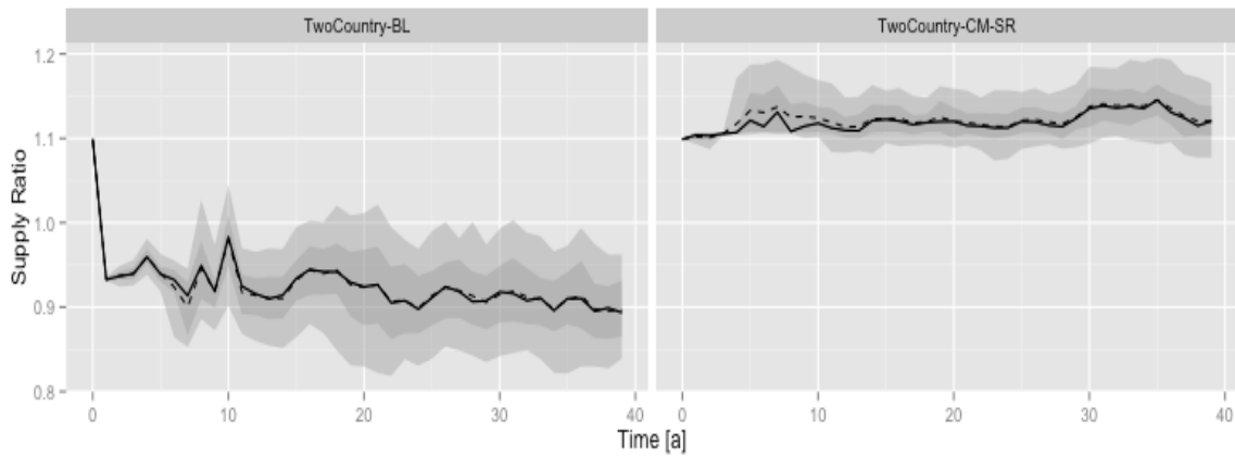
Figure 6.11: Supply ratio in the baseline (left) and in CM-SR scenario (right) in Zone A
