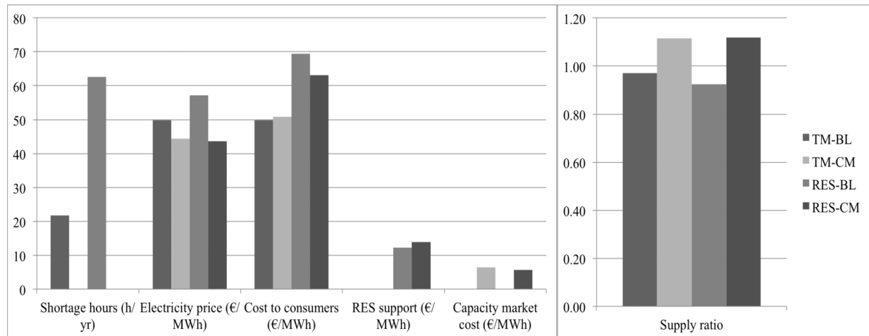
Figure 4.2: Comparison of indicators for the TM and RES scenarios.
