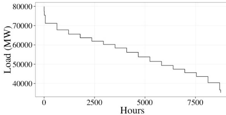
Figure 2.2: Example of a load-duration curve in EMLab-Generation for one country.
