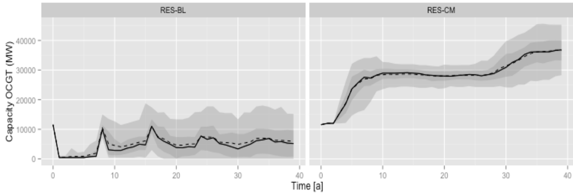
Figure 4.9: OCGT development in presence of high share of renewables
