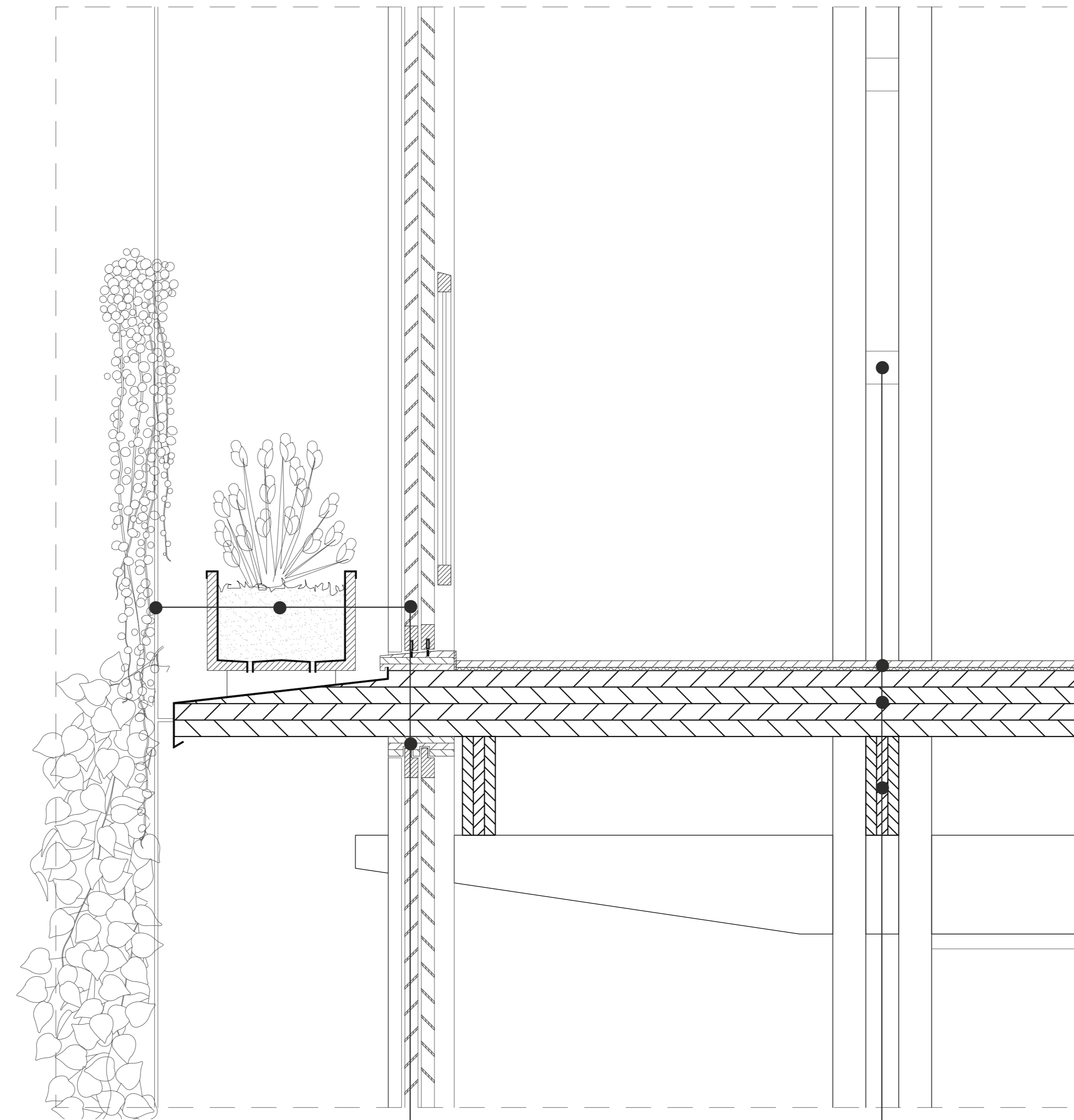
VERTICAL FACADE DETAIL, B
