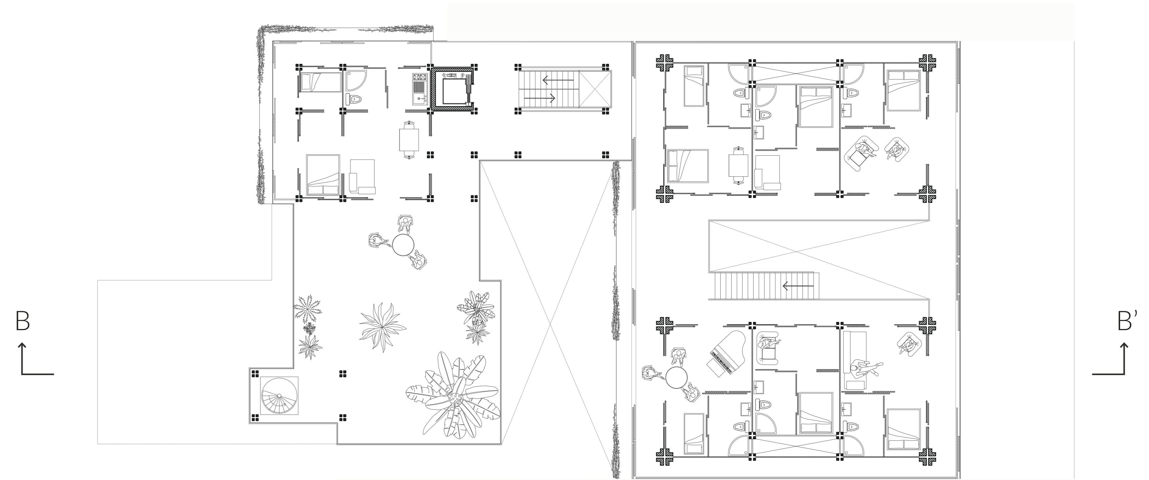
RESIDENTIAL FLOOR PLAN 4 th FLOOR
