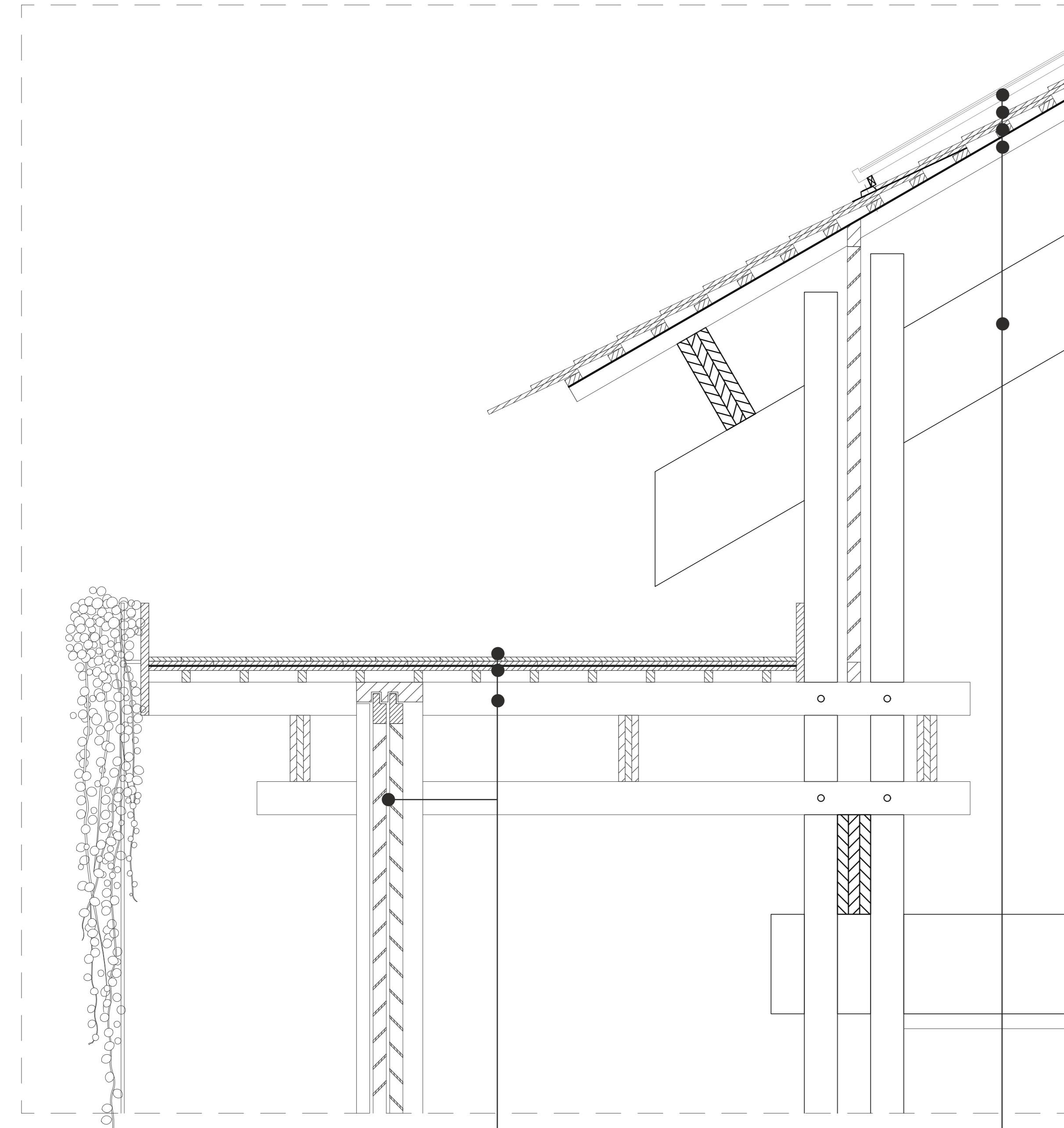
VERTICAL ROOF DETAIL, A
