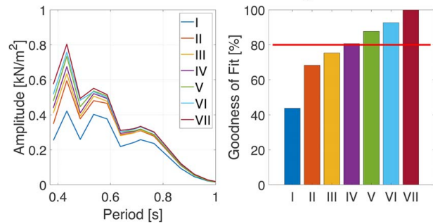
Fig. 5 Results from the convergence study on mean drift loads for the surge direction
