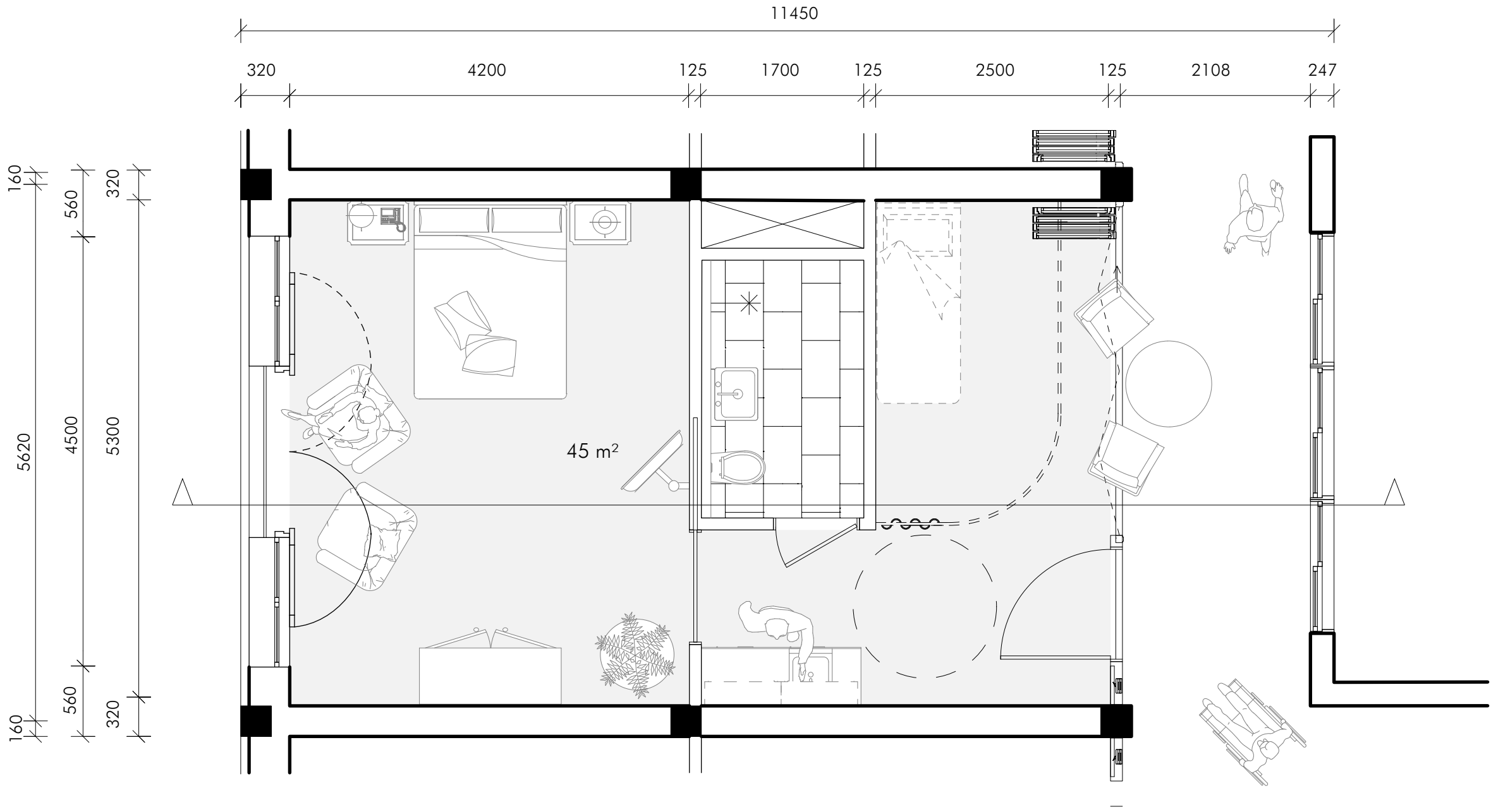
Floor plan 1:50
