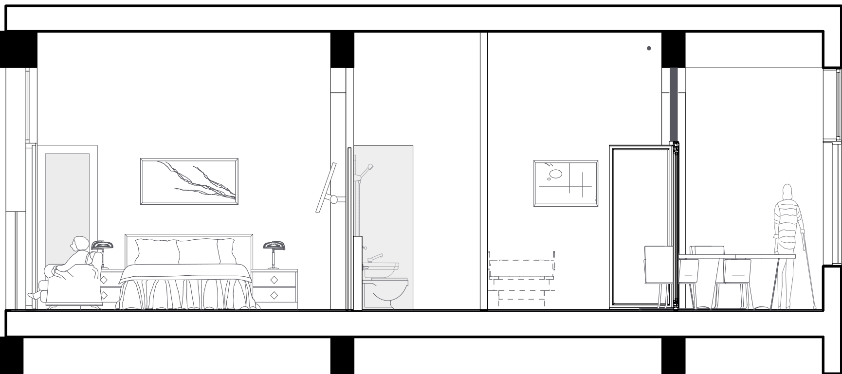
Section 1:50
