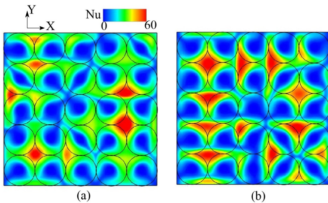
Fig. 9. Instantaneous Nusselt number distribution (top view) at the bottom wall, in a cavity with (a)1 layer (b) 5 layers of spherical beads at 2.3 \times 10^7 obtained with pore-structure resolved (P-R) simulations.
