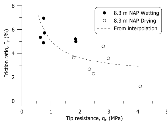
Figure 19. Comparison between the friction ratio from field measurement and the predicted one from harmonic interpolation of tip resistance and sleeve friction
