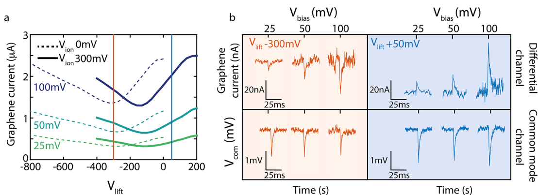
Figure 4. Proof-of-principle. (a) Mapping of the graphene current response to a sweep in V_{\text{lift}} gate potential, at different V_{\text{bias}} (25 mV, green, 50 mV, turquoise, and 100 mV, purple), and for two values of V_{\text{ion}} (0 mV, dotted line, and 300 mV, solid line). The orange and blue lines indicate the V_{\text{lift}} gate potentials at which we measure the pulses displayed in panel b (i.e., V_{\text{lift}} = -300 mV and +50 mV, respectively). (b) Response from the differential current amplifier to -20 mV pulses of 1 ms in V_{\text{ion}} . The positive probe ( V_{\text{ion}} = 300 mV) is located on the graphene side (i.e., trans side) of the membrane. The response in the graphene current is, as expected, different on both sides of the Dirac curve: We observe current dips (orange) for V_{\text{lift}} = -300 mV and current peaks (blue) for V_{\text{lift}} = +50 mV. Measurements were done at three values for the bias voltage, 25, 50, and 100 mV. As expected, larger signals are measured in the graphene current for higher bias voltages. The common mode channel presents the capacitive signals, and as expected, these do not change sign or magnitude, as these do not depend on the gate voltage nor the bias voltage. A signal amplitude of 1 mV corresponds to a current of 200 pA.
