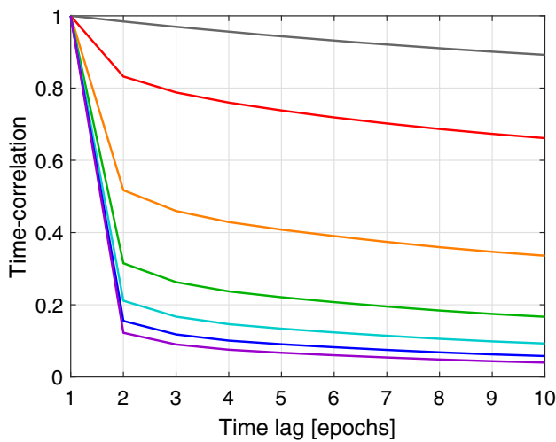
Fig. 8 Time correlation of the estimated between-satellite combined PPP-RTK code corrections as function of time lag with a latency ranging from 0 to 30 s. The results correspond to an individual GPS satellite. The legend of Fig. 7 is applicable here
