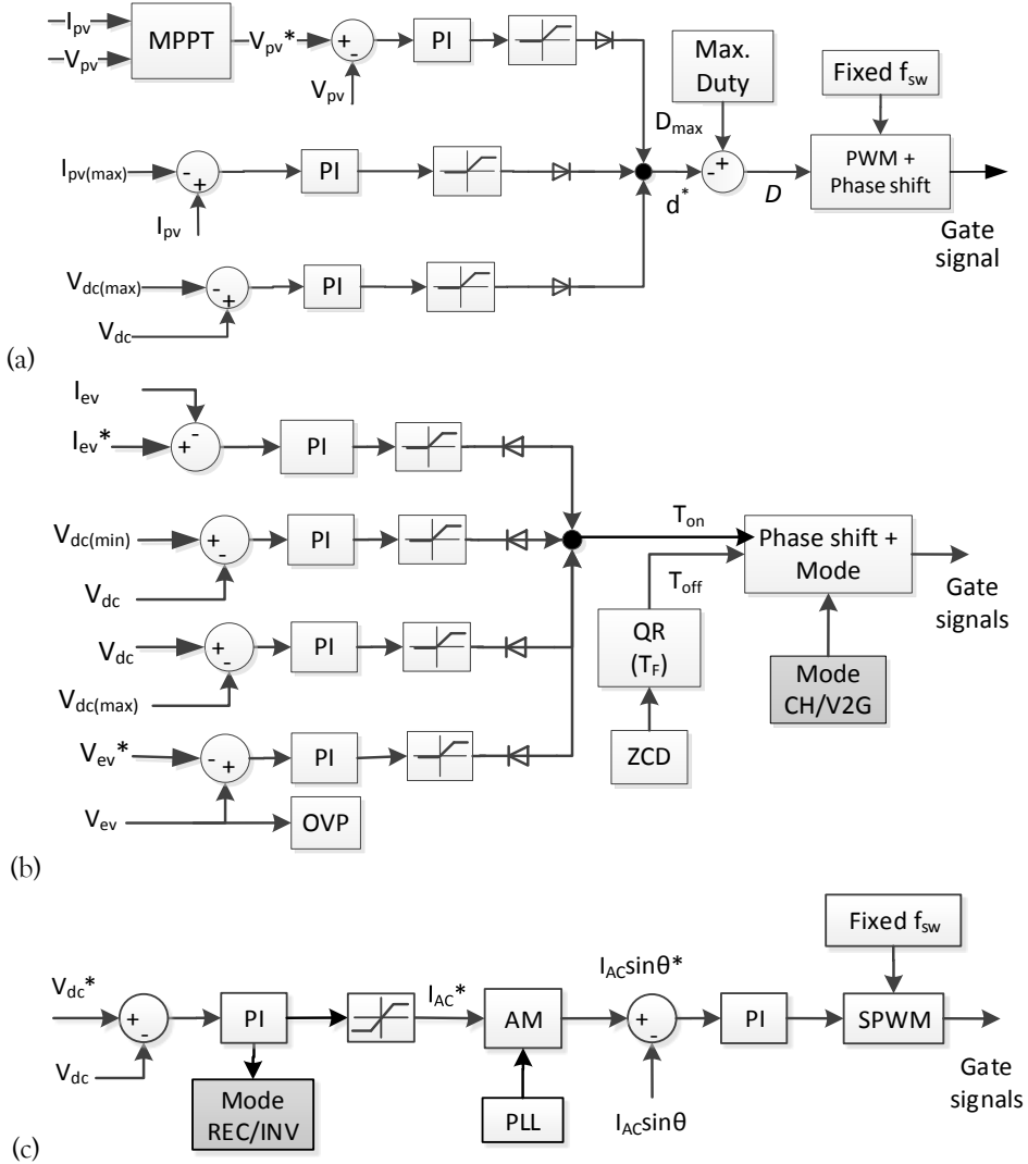
Fig. 5.12. Schematic of the closed loop control: (a) PV converter, (b) EV charger and (c) Grid inverter
