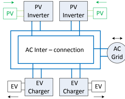
Fig.1.3. Existing solution for solar charging of EV is based on a DC/AC solar inverter to extract PV power and then an AC/DC EV charger is used to charge the EV.
