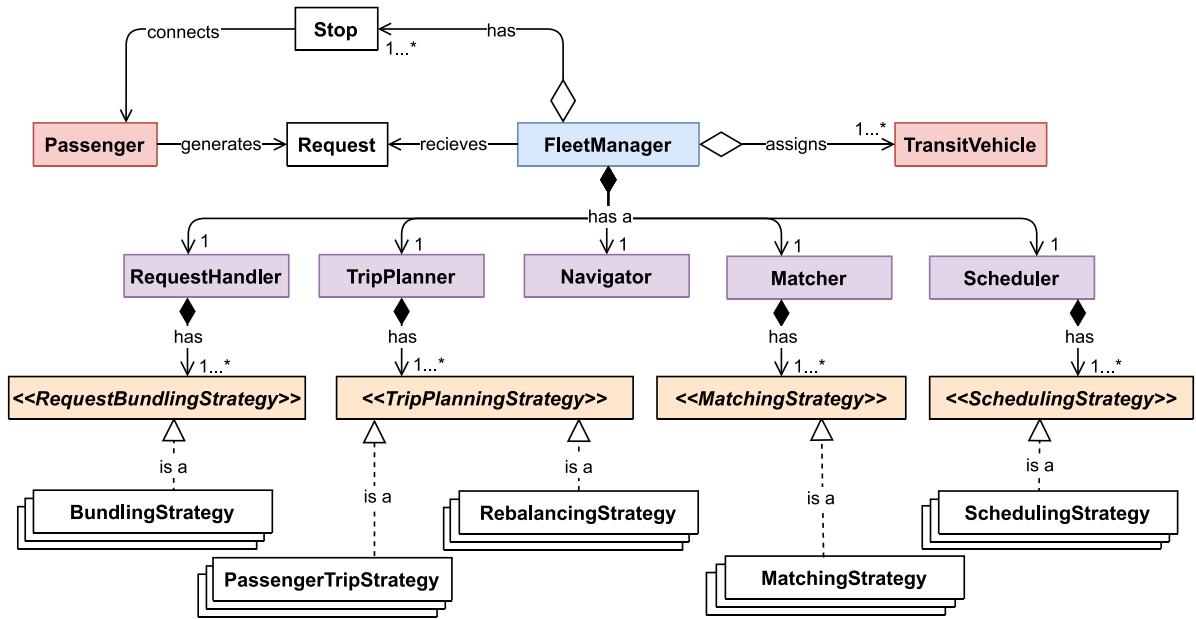
Fig. 2. Class diagram of FleetManager (blue) and member supporting classes (purple), with one or several strategies (orange). Arrows display relationships relevant for connecting Passenger and TransitVehicle agents (red). (For interpretation of the references to color in this figure legend, the reader is referred to the web version of this article.)
