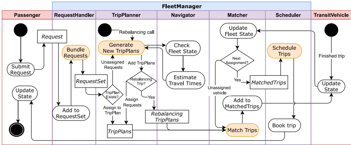
Fig. 3. An activity diagram for greedy vehicle-to-passenger assignment. Column headers and coloring correspond to classes displayed in Fig. 2. Activities are displayed as rounded rectangles, diamonds as conditional branches, and straight rectangles as data structures passed between classes. Orange activities are associated with strategies of the containing class. (For interpretation of the references to color in this figure legend, the reader is referred to the web version of this article.)
