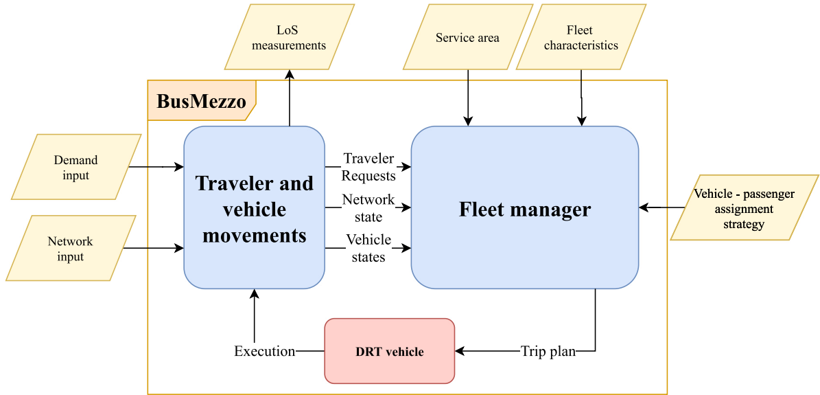
Fig. 1. High-level overview of the public transit simulation framework.
