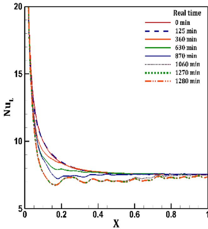
Fig. 10. Local Nusselt number for Da = 10^{-4} and Re = 100 .
