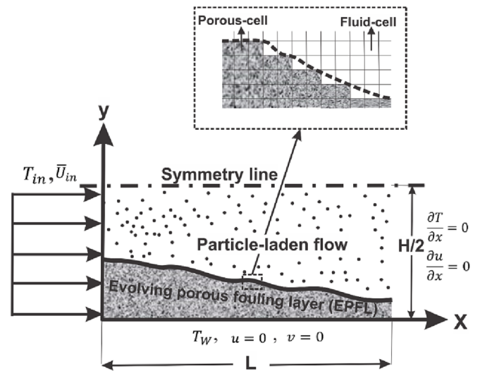
Fig. 1. The schematic of the problem.
