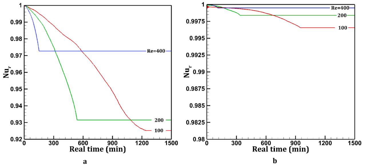
Fig. 12. The variations of the average Nusselt number ratio for different Reynolds numbers and (a) Da = 10^{-4} and (b) Da = 5 \times 10^{-3} .
