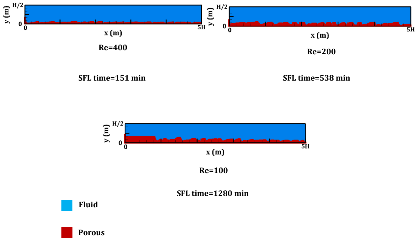
Fig. 16. The SFL profile and SFL time for Da = 10^{-4} and different Reynolds numbers.
