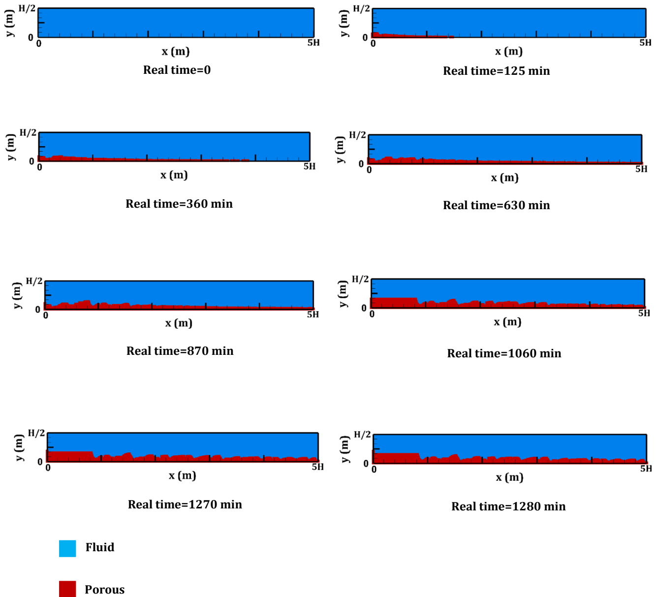
Fig. 8. EPFL generation in duct over the time for Da = 10^{-4} and Re = 100 .
