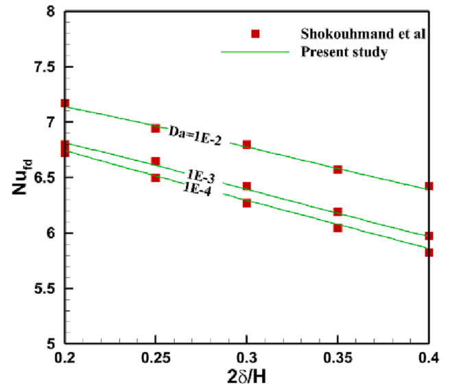
Fig. 6. Validation of the fully developed Nusselt number versus dimensionless FPL thickness for different Darcy numbers.
