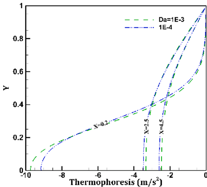
Fig. 15. The thermophoresis acceleration in different sections of the duct at X = 0.2 , X = 2.5 , and X = 4.5 .
