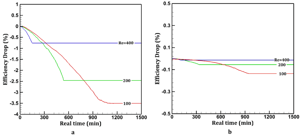
Fig. 14. The thermal efficiency reduction of the duct for various Reynolds numbers and (a) Da = 10^{-4} (b) Da = 5 \times 10^{-3} .
