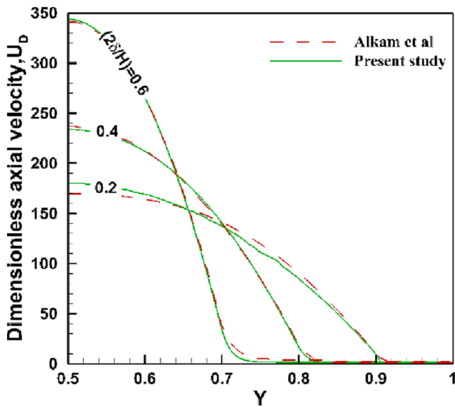
Fig. 5. Validation of dimensionless axial velocity profile against dimensionless vertical coordinate for various FPL thicknesses at X = 2 .
