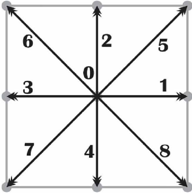
Fig. 2. The schematic of the D_2Q_9 lattice model.
