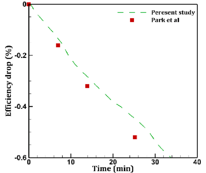
Fig. 7. Validation of the thermal effectiveness reduction over time with that of a real EGR duct.
