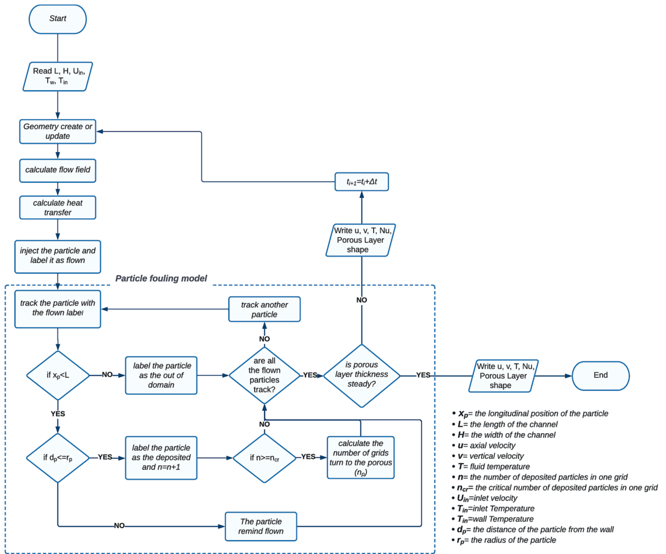
Fig. 3. The flowchart of the fouling growth simulation.
