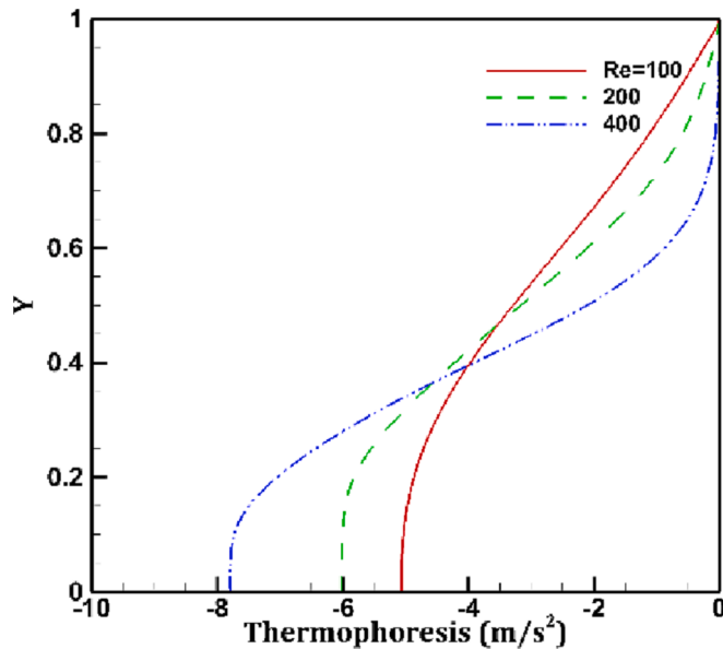
Fig. 17. The y-distribution of the thermophoresis acceleration at X = 1 for different Reynolds numbers.
