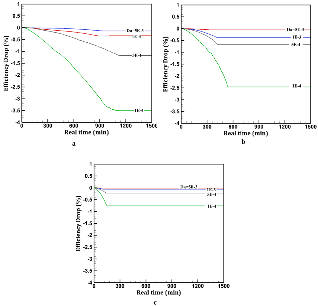
Fig. 13. The thermal efficiency reduction of the duct for various Darcy numbers and (a) Re = 100 , (b) Re = 200 , and (c) Re = 400 .
