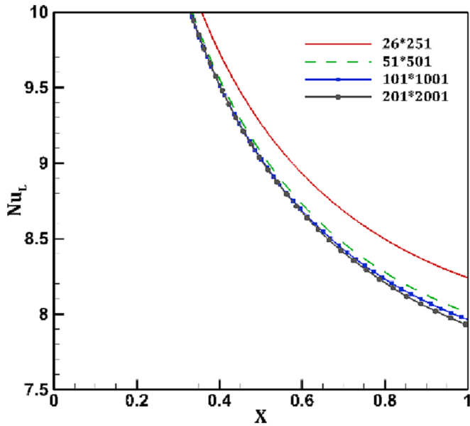
Fig. 4. The results of the local Nusselt number for Da = 5 \times 10^{-3} , Re = 400 , and e = 0.3 .
