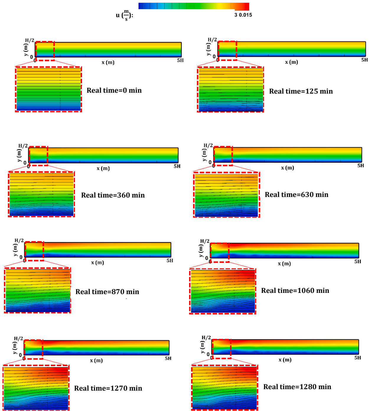
Fig. 9. Velocity contours and streamlines at different times for Da = 10^{-4} and Re = 100 .
