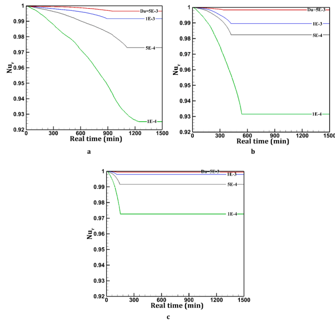
Fig. 11. The variations of the average Nusselt number ratio for different Darcy numbers and (a) Re = 100 , (b) Re = 200 , and (c) Re = 400 .
