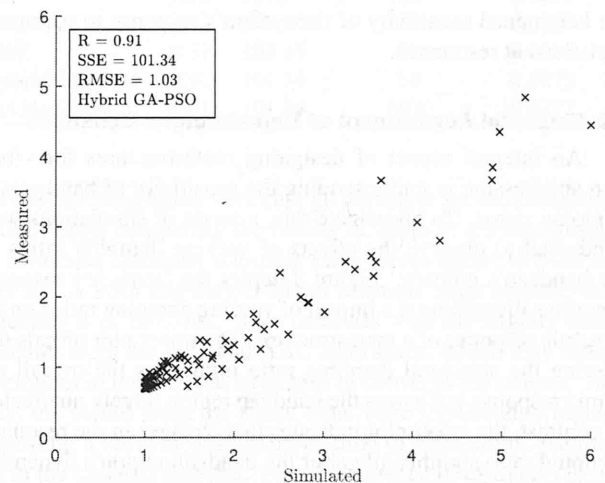
FIGURE 6: Scatter plot comparing measured data to Hybrid GA-PSO simulated estimations, demonstrating the algorithm's efficacy in predicting the structural modal damping ratio ( \zeta_m ) with a correlation coefficient (R) of 0.91.
