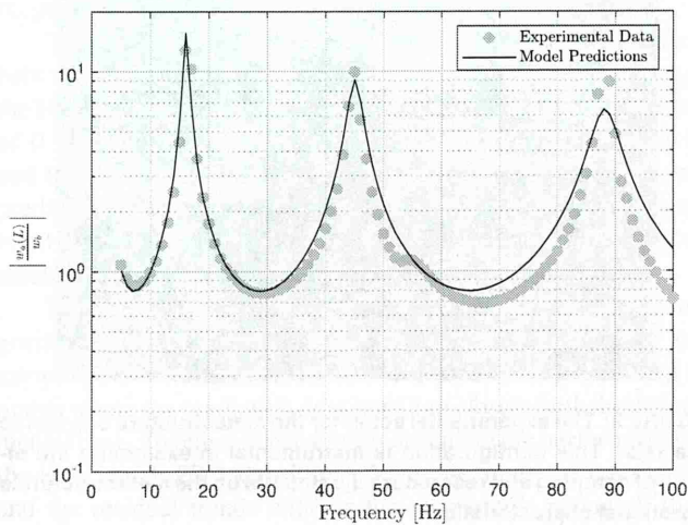
FIGURE 5: Transmittance response of a cantilever beam with Hybrid GA-PSO algorithm estimations, highlighting the model's alignment with experimental data for structural modal damping ratio ( \zeta_m ) estimation.
