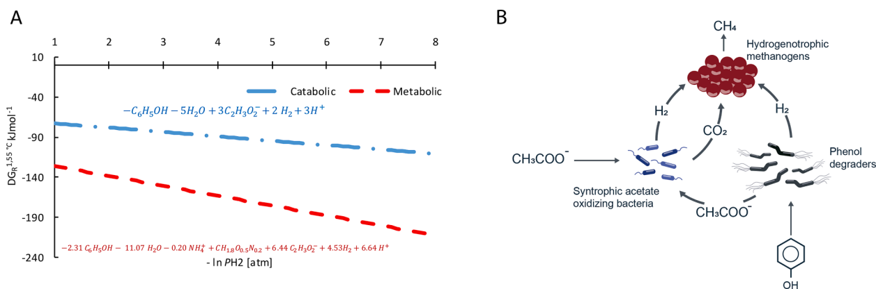
Fig. 6. Effect of the changes in the hydrogen partial pressure ( PH_2 ) on the \Delta G^{1.55^\circ C} (correction for temperature and reagents concentration) of the catabolic (blue) and metabolic reactions (red) of phenol degradation under thermophilic anaerobic conditions. The metabolic equation considers a microorganism capable of the anaerobic degradation of phenol to acetate and hydrogen (A). Scheme for the proposed syntrophic association for phenol degradation under thermophilic anaerobic conditions between phenol degraders, syntrophic acetate oxidizing bacteria (SAOB) and hydrogenotrophic methanogens. (For interpretation of the references to colour in this figure legend, the reader is referred to the web version of this article.)
