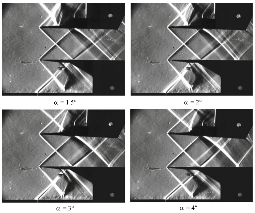
Fig. 40 Schlieren visualizations for a fixed flat plate location at X = 0.9\text{ mm} . Effect of the impinging shock intensity— Re_{X_I} \approx 0.61 \times 10^6
