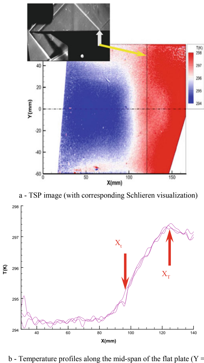
Fig. 39 Temperature Sensitive Paint measurements. a —TSP image (with corresponding Schlieren visualization). b —Temperature profiles along the mid-span of the flat plate ( Y = 0 )
