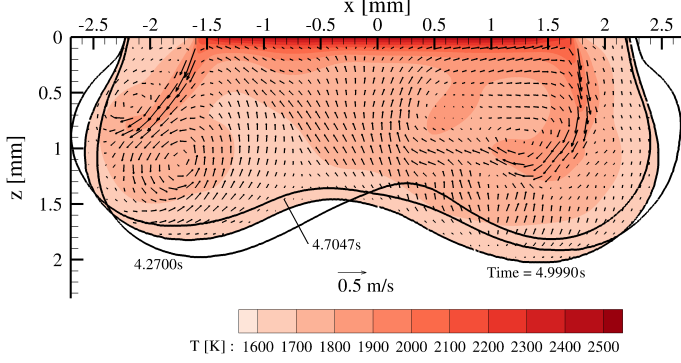
Figure 6: Melt pool shape, temperatures (in Kelvin) and velocity vectors in the y=0 mm plane at the end of heating t = 5.0 s. Note that the velocity vectors have been interpolated to a coarse grid in post-processing for clarity. The pool shape at two other time instances is overlaid, showing the pool boundary oscillation.
