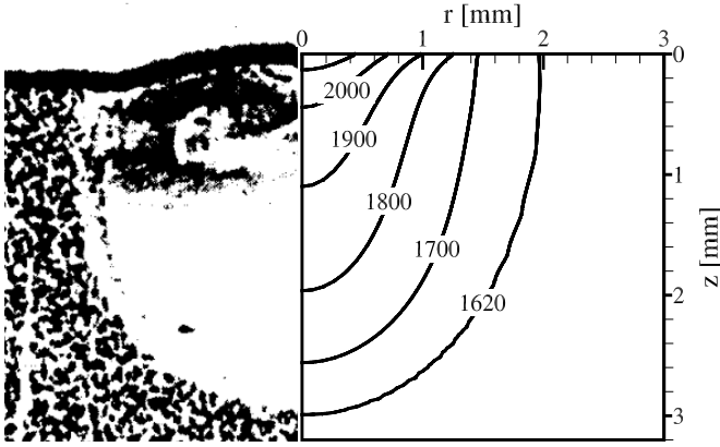
Figure 5: The right hand side of the figure shows the current faithful representation of the experimental result (left half of the figure, reproduced from [7] with permission of the publisher, sized to match scale on the right) after 5 s of welding, using an enhancement factor of 7 for both the viscosity and the thermal conductivity. Temperature isolines in Kelvin (simulation result, right half).
