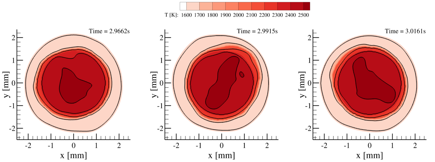
Figure 9: Pool surface ( z=0 mm) temperatures in Kelvin at three time instances, top view. Isolines are drawn at 1620K, 1700K, 2200K, 2400K and 2500K (from outside to inside).
