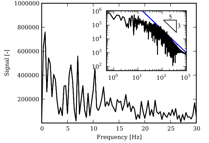
(a) DFT of temperature at monitoring point
