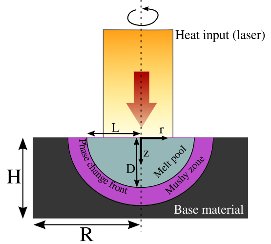
Figure 1: Schematic representation of the studied laser welding.
