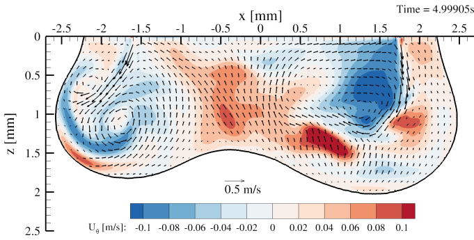
Figure 7: In-plane ( x,z ) velocities in the y=0 mm plane at t = 5.0 s indicated by vectors, and out-of-plane (azimuthal) velocities indicated by colour contours.
