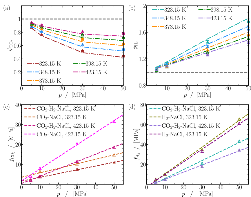
Figure 11. Fugacity coefficients and fugacities of CO 2 and H 2 in the CO 2 -H 2 -NaCl brine system computed from MC simulations using eq 6. Fugacity coefficients of (a) CO 2 and (b) H 2 in the gas-rich phase compared to predictions from REFPROP 108 based on the gas-phase compositions from MC simulations depicted by dashed lines. (c,d) Fugacities of CO 2 and H 2 computed from eq 13 using fugacity coefficients from (a,b), respectively. The dashed lines are linear fits to the data points. The open symbols represent fugacities computed for CO 2 and H 2 in the respective binary systems of CO 2 -NaCl and H 2 -NaCl, respectively. The raw data of the fugacity coefficients are provided in Table S7 of the Supporting Information.
