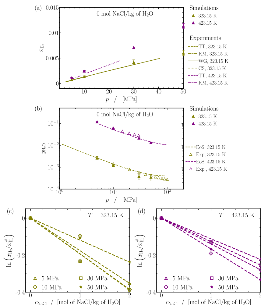
Figure 10. (a) Comparison of simulations (symbols) with experimental (lines) predictions for \text{H}_2 solubilities in pure \text{H}_2\text{O} . Experimental studies of Torin Ollarves and Trusler (TT), 79 Kling and Maurer (KM), 172 Wiebe and Gaddy (WG), 173 and Chabab et al. (SC) 57 are considered for the comparison. (b) Comparison of the water content in the gas phase between our simulations and the experiments from Torin Ollarves and Trusler (TT). Predictions from the equation of state from Torin Ollarves and Trusler (TT) are also plotted alongside. (c,d) Reduction in the solubility of \text{H}_2 as a function of NaCl concentration in brine. The logarithm of the ratio of \text{H}_2 solubility in brine to its solubility in pure water is plotted against NaCl concentration. Linear fits to the data are shown as dashed lines. The raw data of the solubilities are provided in Table S5 of the Supporting Information.
