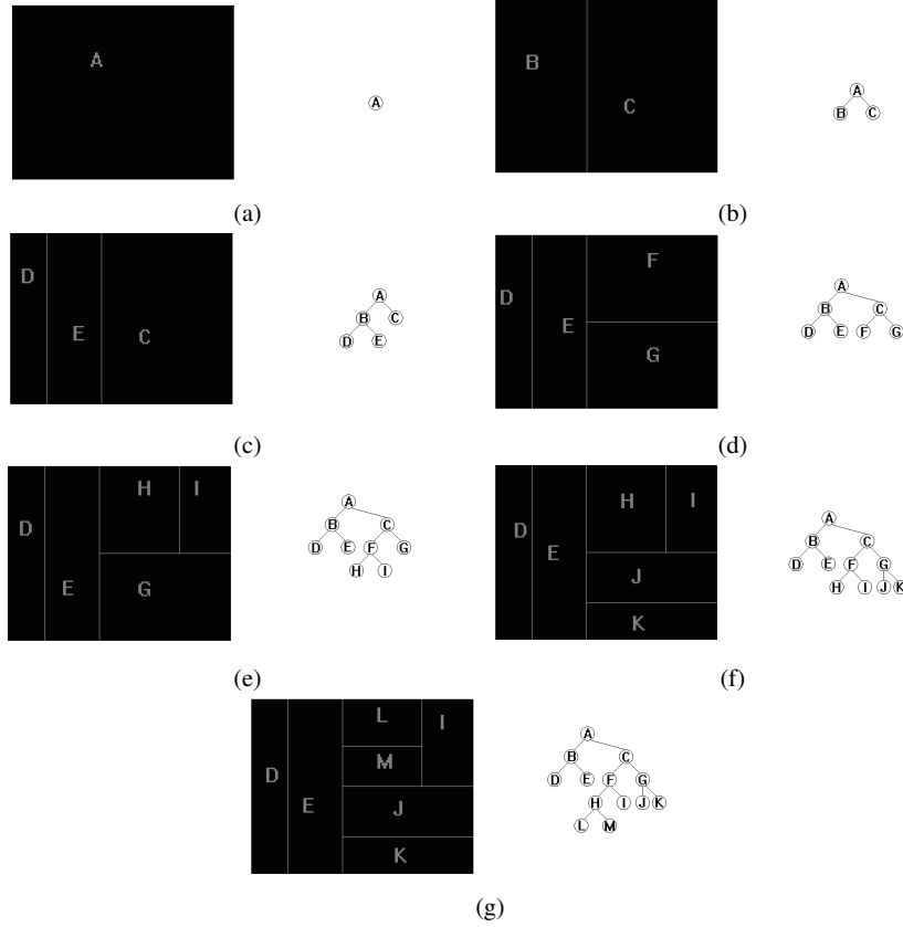
Fig. 3.3: Stochastically partitioning the dungeon area A, which is contained in the root node of the BSP tree. Initially the space is split into B and C via a vertical line (its x -coordinate is determined randomly). The smaller area B is split further with a vertical line into D and E; both D and E are too small to be split (in terms of width) so they remain leaf nodes. The larger area C is split along a horizontal line into F and G, and areas F and G (which have sufficient size to be split) are split along a vertical and a horizontal line respectively. At this point, the partition cells of G (J and K) are too small to be split further, and so is partition cell I of F. Cell H is still large enough to be split, and is split along a horizontal line into L and M. At this point all partitions are too small to be split further and dungeon partitioning is terminated with 7 leaf nodes on the BSP tree. Figure 3.4 demonstrates room and corridor placement for this dungeon.
